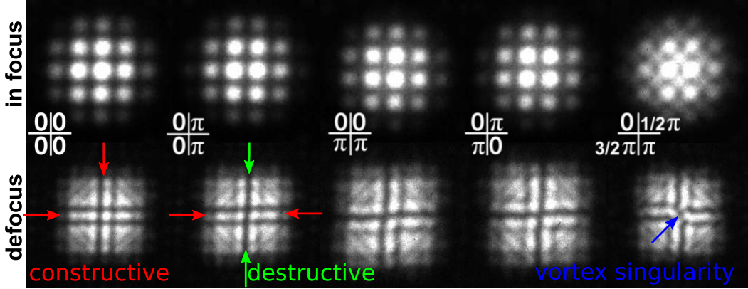
Fig. 3. (top row) Set of diffraction pattern for 5 different applied potential configurations leading to an approximate realisation of the phase symmetry as indicated on each panel. (bottom row) Defocused diffraction patterns for the same potential configuration showing more directly the constructive and destructive interference features between the 4 patches as indicated by arrows.
