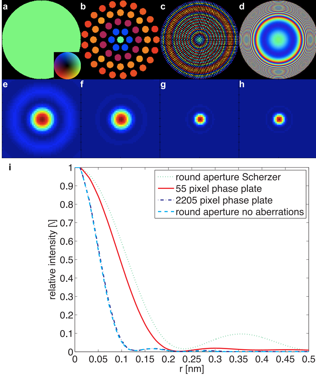
Fig. 5. Simulated performance of a programmable phase plate as a C_s corrector assuming 300 keV and C_s=1 mm. Two phase plates are simulated, a modest 55 pixel plate and a more demanding 2205 pixel phase plate. The defocus of the lens system was optimised to -75 nm and -250 nm respectively to reach the optimum probe shape. The result is compared to an ideal aberration free system with the same round aperture with opening angle 20 mrad. The resulting probe intensities are shown respectively in (e,f,g,h), the images have dimension 1x1 nm. The azimuthally averaged probe intensity is shown in (i). Note that the low pixel count phase plate in (b) does not significantly improve the probe size but does improve the tails. Introducing significantly more pixels (c) approaches the ideal case quite closely. Note that even though the probe appears similar to the ideal diffraction limited case (d), a significant amount of the probe intensity is scattered to higher angles due to the narrow pixel shape function which would lead to an increased background when using this probe for imaging. The colorwheel shown as inset in (a) shows the colorscale used in (a,b,c,d) to depict both amplitude as intensity and phase as hue.
