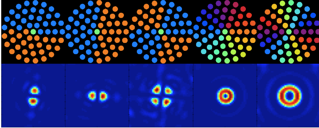
Fig. 6. A series of exotic electron beams prepared with a modest programmable phase plate (55 pixels, 41% fill-factor) approximating (from left to right) HG_{0,1} , HG_{1,0} , HG_{1,1} , LG_{0,1} , LG_{0,2} . This shows that even a modest programmable phase plate can be very useful for producing exotic beam types that were hitherto difficult to produce in a TEM requiring time consuming and static (holographic) phase plates.
