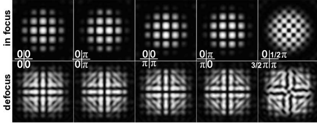
Fig. 4. Simulated diffraction patterns assuming an ideal programmable phase shifting device with dimensions matching the experiment. Note the strong similarity in the intensity patterns for both in focus (top row) and defocused diffraction pattern series.
