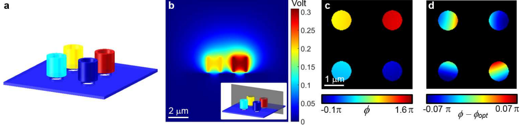
Fig. 2. Simulated potential of the setup (a) showing the four electrodes at different potential of 0, 103, 206, 309 mV in order to obtain 0, 1/2\pi , \pi , 3/2\pi phase shift. A slice through 2 neighbouring electrodes (b) shows the potential homogeneity inside the cylinders with fringe fields extending above the electrodes due to the missing top ground plane. The projected potential is shown in (c) in units of phase shift assuming 300 kV electrons. The difference with the intended phase plate of 0, 1/2\pi , \pi , 3/2\pi is shown in (d) with a maximum deviation that remains below 0.07\pi as a result from the cross talk between the neighbouring pixels due to the lack of a top ground plane.
