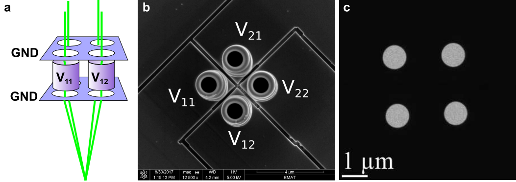
Fig. 1. (a) sketch of an array of weakly excited electrostatic einzel lenses individually controlling the phase of 4 electron beams which recombine in the far field to form a programmable interference pattern. (b) SEM image of a proof of concept implementation of a 2x2 phase plate prepared as described in this paper. (c) TEM image of the aperture showing the geometry of the 4 aperture holes as well as the limited fill factor.
