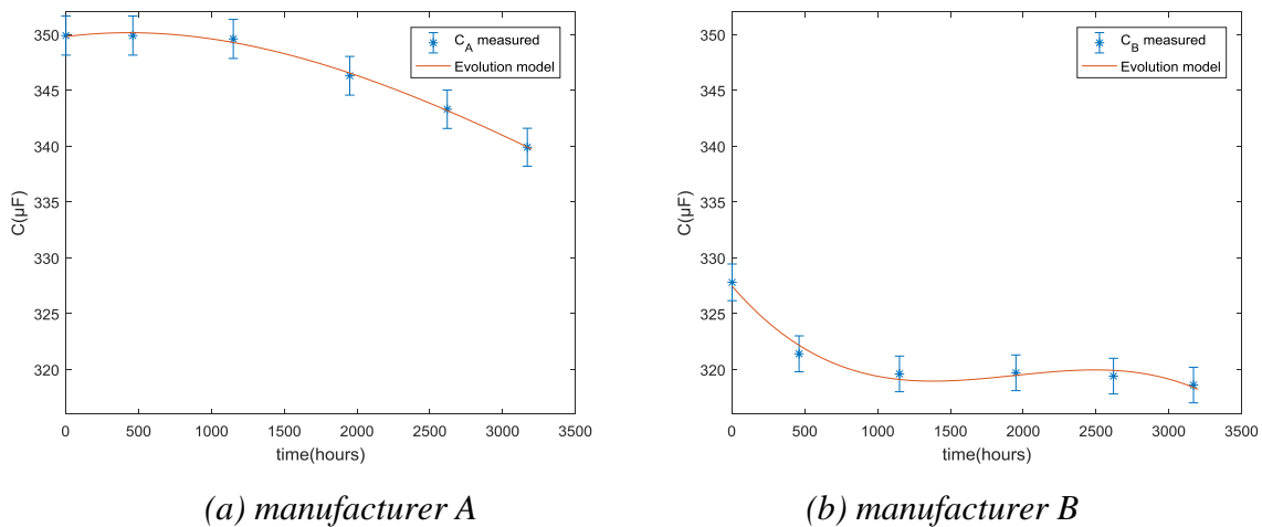
Figure 4 Evolution of C with time – test c(85 ; 500)
