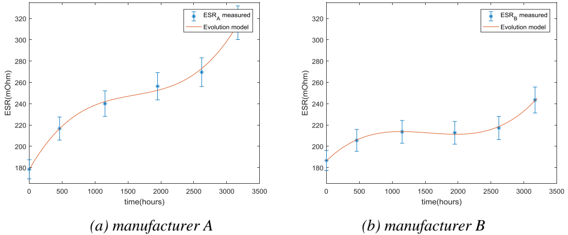
Figure 2 Evolution of ESR with time – test c(85 ; 500)
