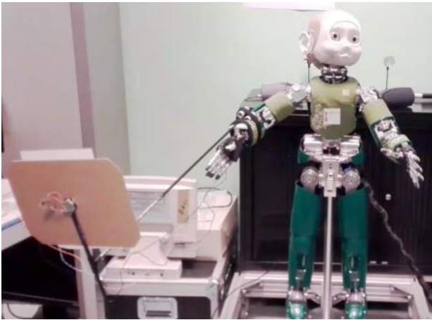
Fig. 1. The iCub humanoid robot with the recording device fixed on its right arm. The device consists of a rod ended with a loudspeaker embedded into a visual marker for video tracking.
