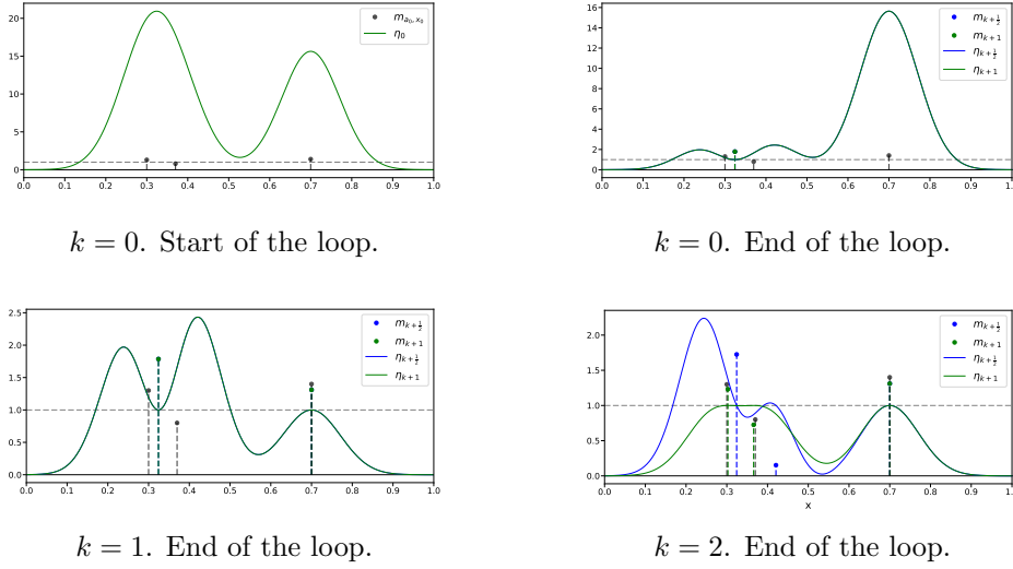
Figure 7: Main steps of the SFW algorithm.
