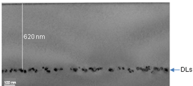
FIG. 1. TEM cross-section image showing dislocation loops introduced in Si after implantation with 2 \times 10^{15} \text{ Ge cm}^{-2} and annealed at 1000 °C for 15 s.
