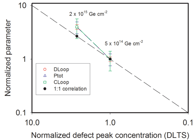
FIG. 11. Normalised defect properties ( D_{tot} , C_{tot} , or P_{tot} ) as a function of defect peak concentration extracted from DLTS for the hole trap H(0.25) in the samples implanted with 5 \times 10^{14} Ge cm -2 or 2 \times 10^{15} Ge cm -2 annealed at 1050 °C or 1000 °C, respectively.
