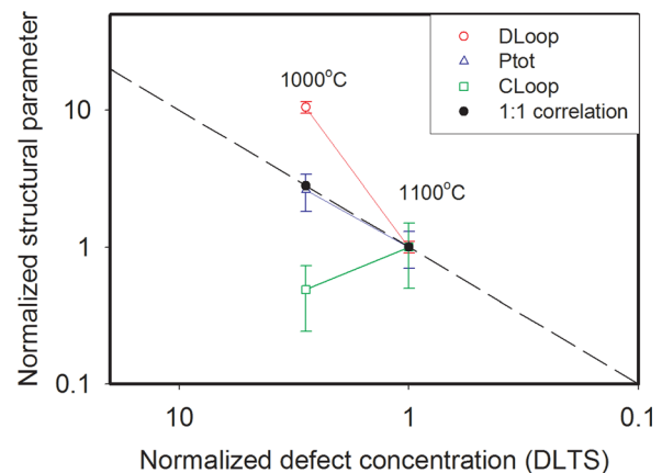
FIG. 12. Normalised defect properties ( D_{tot} , C_{tot} , or P_{tot} ) as a function of defect peak concentration extracted from DLTS for the electron trap E(0.38) in samples implanted with 2 \times 10^{15} Ge cm -2 annealed at 1000 °C or 1100 °C.
