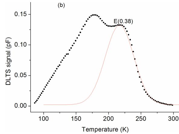
FIG. 4. DLTS spectra of electron traps in the sample implanted with 2 \times 10^{15} Ge \text{cm}^{-2} and annealed at (a) 1000 °C for 15 s and (b) 1100 °C for 300 s. The experimental data are shown in solid circles, whereas the fit by the energy band model is indicated by solid lines.
