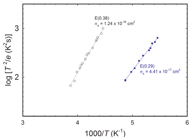
FIG. 3. Arrhenius plots for the defects introduced by implantation of 2 \times 10^{15} Ge \text{cm}^{-2} into n-type Si from which activation energies and “apparent” electron capture cross sections were extracted.
