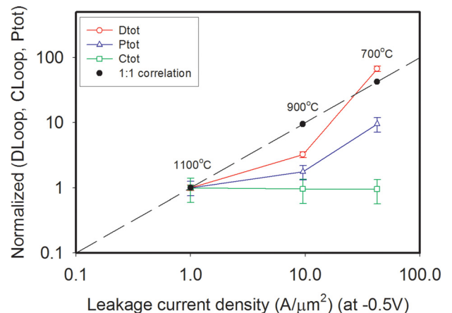
FIG. 19. Normalised defect properties ( D_{tot} , C_{tot} , or P_{tot} ) as a function of leakage current for the n^+p diodes with EOR in the neutral region.
