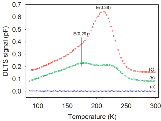
FIG. 2. DLTS spectra in n-type Si for the (a) reference sample and after implantation to a dose of 2 \times 10^{15} Ge \text{cm}^{-2} and annealing at (b) 1100 °C for 300 s and (c) 1000 °C for 15 s.
