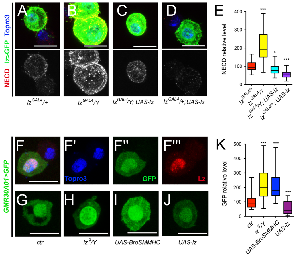
Fig 9. Lz represses Notch expression. (A-D) Immunostainings against NECD (Notch extracellular domain) in blood cells from lz-GAL4, UAS-mCD8-GFP/+ (A), lz-GAL4, UAS-mCD8-GFP/Y (B), lz-GAL4, UAS-mCD8-GFP/Y; UAS-lz (C) and lz-GAL4, UAS-mCD8-GFP/+; UAS-lz (D) third instar larvae. NECD immunostaining only is shown in the lower panels. Nuclei were stained with Topro3. (E) Corresponding quantifications of NECD in lz>GFP + blood cells. (F-F''') Immunostaining against Lz in circulating blood cells from Notch GMR30A01 -GAL4, UAS-GFP larvae. Nuclei were stained with Topro3. (F'-F'''): single channel images. (G-J) Notch GMR30A01 -GAL4 -driven expression of GFP in circulating blood cells from larvae of the indicated genotypes. (K) Corresponding quantifications of the level of GFP. (A-D, F-J) Scale bar: 10µm. (E, K) *: p-value<0.05, *** p-value<0.001.
