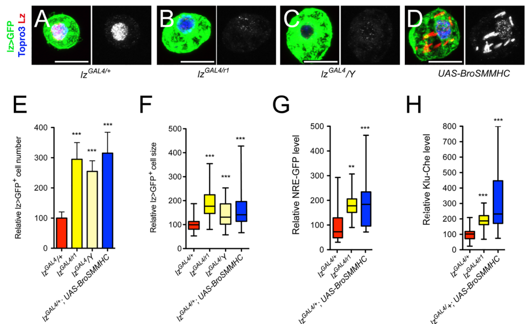
Fig 8. High levels of Lz prevent lz>GFP^+ cell accumulation and Notch signaling overactivation. (A-D) Fluorescent immunostainings of Lz in circulating blood cells from lz^{GAL4} , UAS-mCD8-GFP/+ (A, control), lz^{GAL4} , UAS-mCD8-GFP/lz^{r1} (B), lz^{GAL4} , UAS-mCD8-GFP/Y (C) and lz^{GAL4} , UAS-mCD8-GFP/+ ; UAS-BroSMMHC (D) third instar larvae. Nuclei were stained with Topro3. Scale bar: 10 \mu m. Lz immunostaining only is shown in the right panels. (E-H) Quantifications of lz>GFP^+ cell number (E) and size (F) as well as NRE-GFP (G) and Klu-Cherry (H) expression levels in third instar larvae of the indicated genotypes. **: p-value<0.01, *** p-value<0.001.
