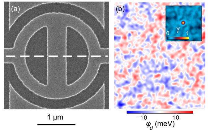
FIG. 2. (a) Scanning electron micrograph of the fabricated sample in an InGaAs/InAlAs heterostructure. (b) Computed real-space disorder potential \varphi_d at the level of the 2DEG that will be used in the forthcoming simulations. The disorder standard deviation S_d is 4.78 meV, calculated taking into account a distribution of Si ionized dopants located 20 nm above the 2DEG (i.e., the thickness of the InAlAs spacer). The inset in (b) shows a map of the autocorrelation as the correlation lag becomes a vector in the x - y plane.
