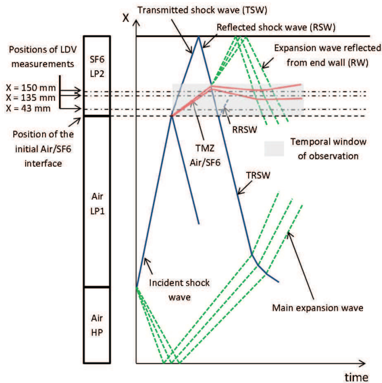
Fig. 10. Schematic (X - t) diagram of an Air/ \text{SF}_6 experiment. Except for the previously defined TMZ acronym, letters W, T and R used in the acronyms refer to 'wave', 'transmitted' and 'reflected' respectively.
