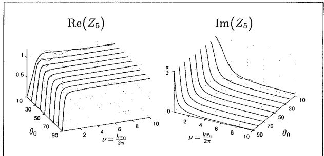
Figure 8. Impedance averaged on S_0 (...) and second order model Z_5 (-).
