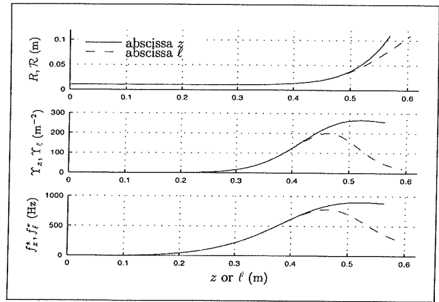
Figure 2. Comparison of the z -models R , Y_z = R''/R , f_z^+ = c\sqrt{Y_z}/(2\pi) , (-) to the \ell -models \mathcal{R} , Y_\ell = \mathcal{R}''/\mathcal{R} , f_\ell^+ = c\sqrt{Y_\ell}/(2\pi) , (- -) for the toy-profile (A1) in appendix A1.
