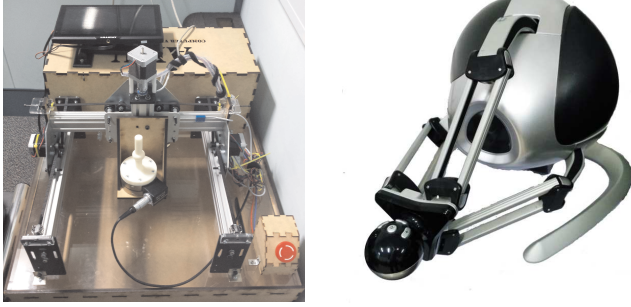
Fig. 5. Master haptic devices used in this paper. A custom made admittance and a COTS NOVINT Falcon joystick.
