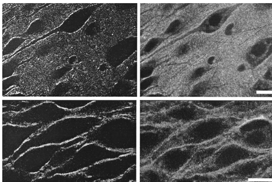
FIGURE 7 (Top panels) Simultaneous 2HG (left) and 2PEF (right) images of a hippocampal slice culture labeled with RH237. Three images were averaged, each with 10 \mu\text{s} pixel integration time and no polarization rotation. Note the enhanced 2HG contrast of the CA1 pyramidal cell walls. (Bottom panels) Non-averaged images of the pyramidal layer in the same slice. The slice was <100 \mu\text{m} thick. The laser power at the sample was <5 mW. Scale bars are 15 \mu\text{m} .
