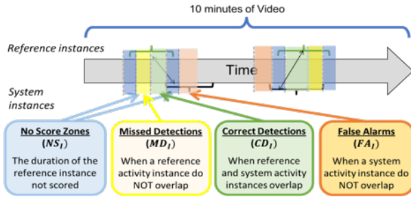
Figure 21: Confusion matrix computation of instance-pairs for temporal localization
