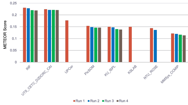
Figure 36: VTT: Comparison of all runs using the METEOR metric
