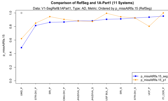
Figure 24: Performance comparison of RefSeg and EvalPart1 on the AD task
