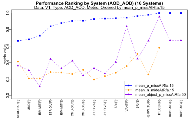
Figure 23: The ranked list of performance (AOD)
