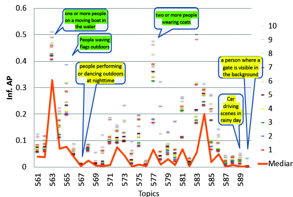
Figure 6: AVS: Top 10 runs (xinfAP) by query number (fully automatic)
