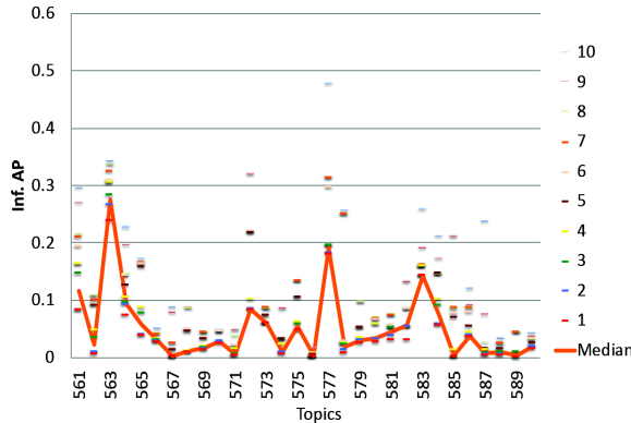
Figure 5: AVS: Top 10 runs (xinfAP) by query number (manually assisted)
