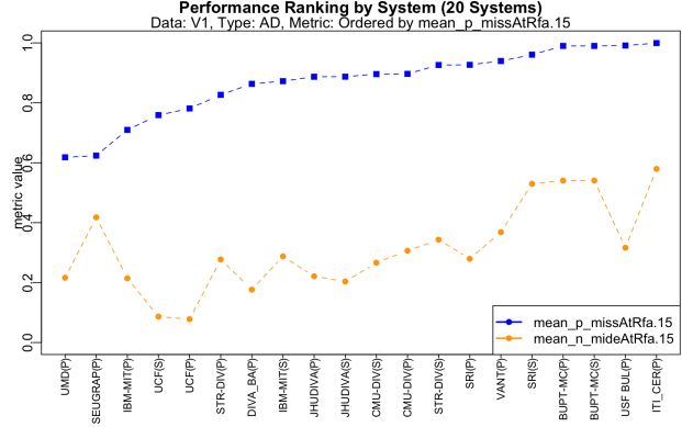
Figure 22: The ranked list of performance (AD)
