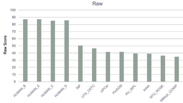
Figure 39: VTT: Average DA score for each system. The systems compared are the primary runs submitted, along with 4 manually generated system labeled as HUMAN_B to HUMAN_E
