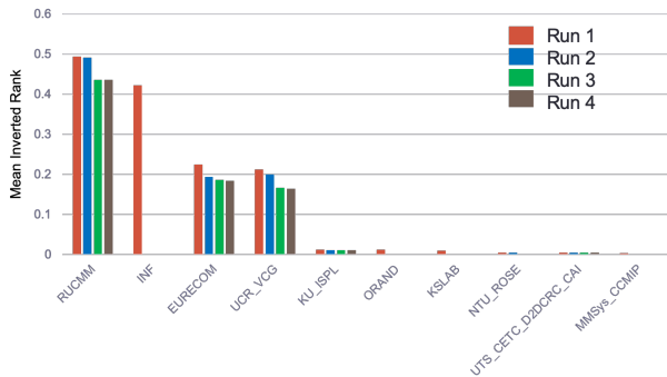
Figure 31: VTT: Matching and Ranking results across all runs for Set D
