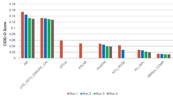
Figure 35: VTT: Comparison of all runs using the CIDEr-D metric
