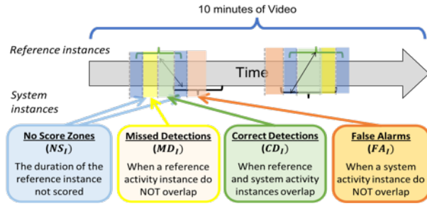
Figure 21: Confusion matrix computation of instance-pairs for temporal localization
