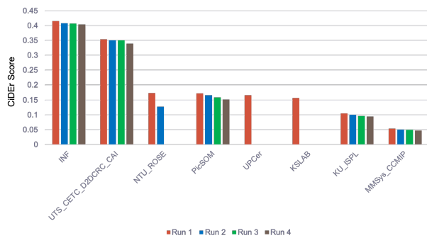
Figure 34: VTT: Comparison of all runs using the CIDEr metric
