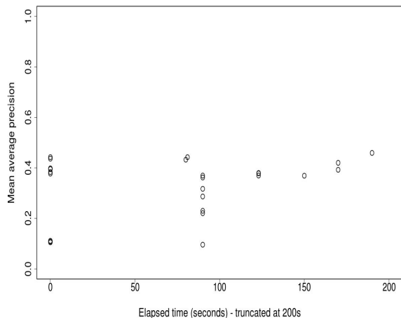
Figure 18: INS: Mean average precision versus time for fastest runs
