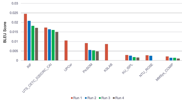
Figure 37: VTT: Comparison of all runs using the BLEU metric
