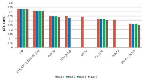
Figure 38: VTT: Comparison of all runs using the STS metric
