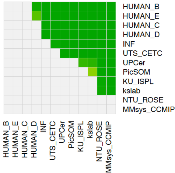
Figure 41: VTT: Comparison of systems with respect to DA. Green squares indicate a significantly better result for the row over the column
