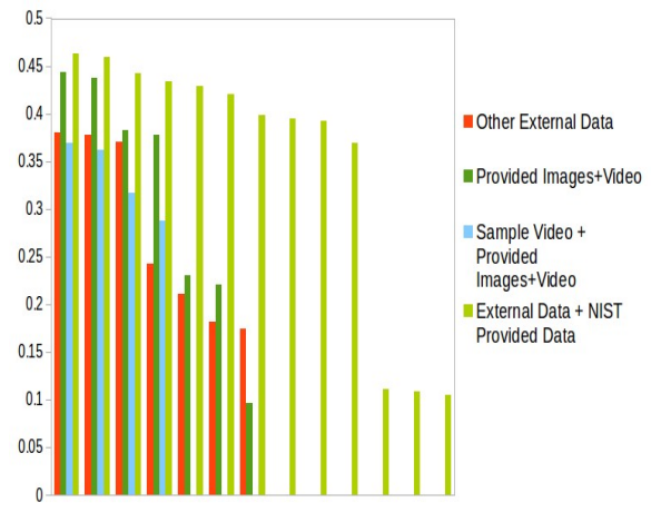
Figure 20: INS: Effect of data source used
