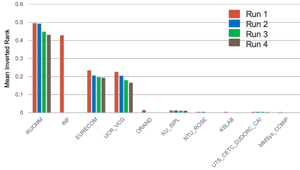
Figure 30: VTT: Matching and Ranking results across all runs for Set C
