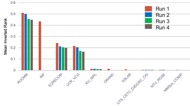
Figure 32: VTT: Matching and Ranking results across all runs for Set E
