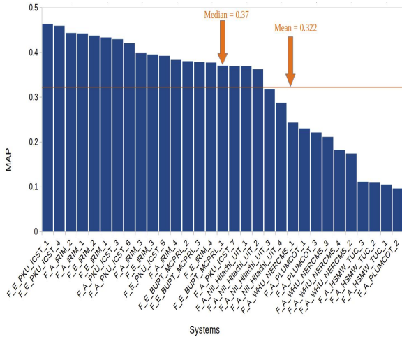
Figure 12: INS: Mean average precision scores for automatic systems
