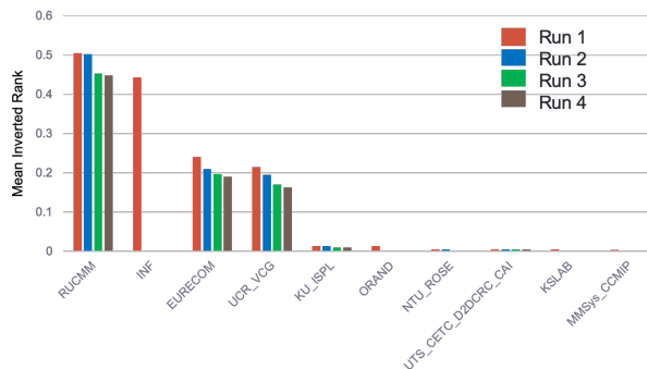
Figure 29: VTT: Matching and Ranking results across all runs for Set B
