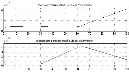
Fig.5 reconstructed inputs F_u , F_p from outputs T_u , T_p in CASE B
