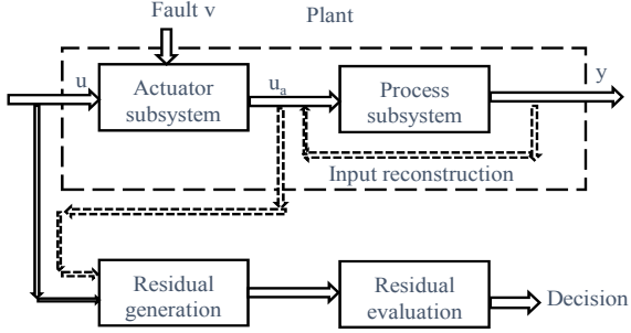
Fig. 1 System structure and FDI algorithm
