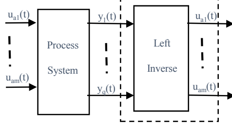
Fig. 2. Input reconstruction
