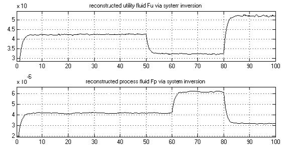
Fig.3 reconstructed inputs F_u, F_p from outputs T_u, T_p in CASE A
