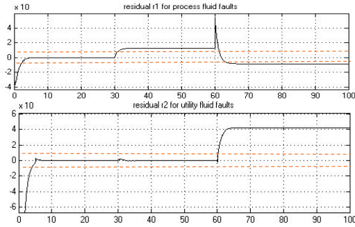
Fig.6 detection and isolation residual in CASE B
