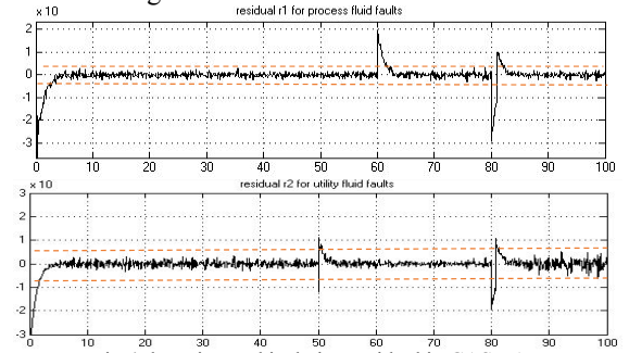
Fig.4 detection and isolation residual in CASE A
