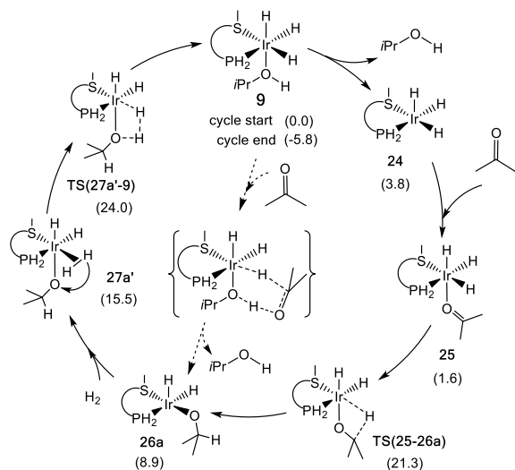
Figure 5. Best cycle for acetone hydrogenation catalyzed by [IrH_4(\mathbf{1}^{Ph})(iPrOH)] ( 9 ). For each species the Gibbs energy in kcal/mol is given in parentheses below the compound symbol.
