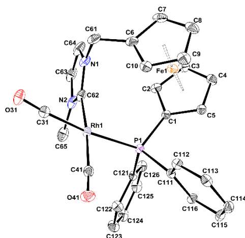
Figure 2. ORTEP representation of the cation in the dicarbonyl complex 2 . Ellipsoids are shown at the 30% probability level. All hydrogen atoms are omitted for clarity.
