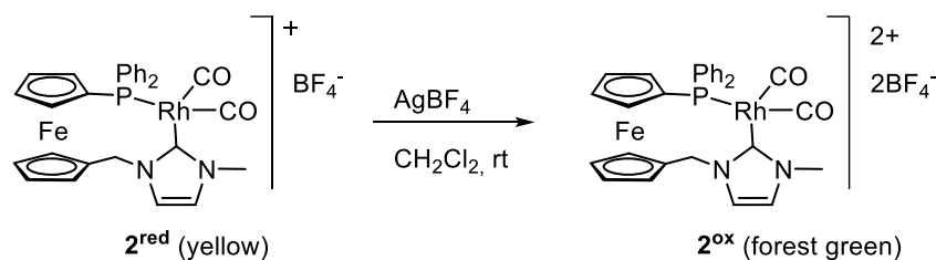
Scheme 3. Oxidation of rhodium(I) carbonyl complex 2 with \text{AgBF}_4 in \text{CH}_2\text{Cl}_2 .
