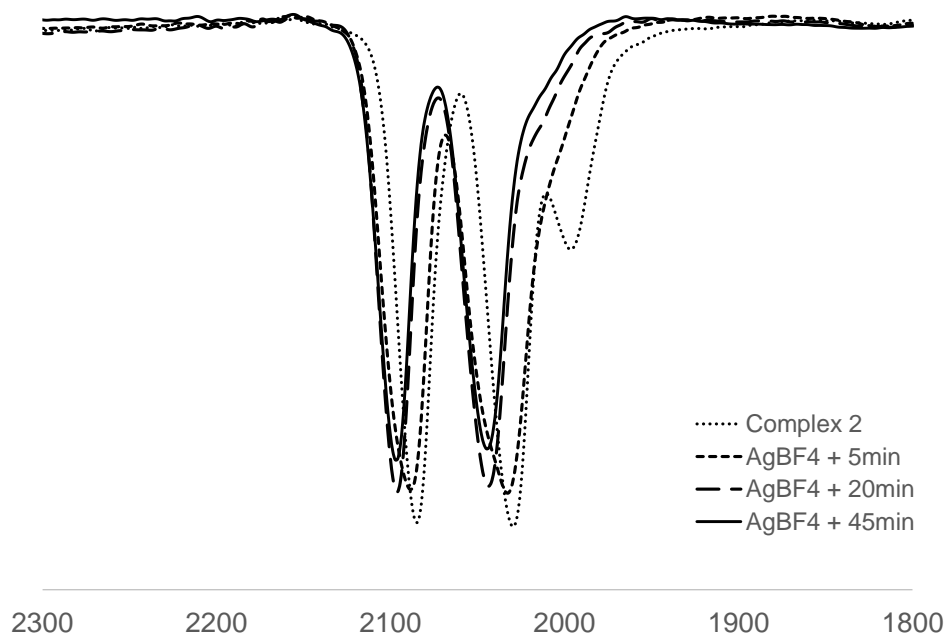
Figure 5. IR spectra (ATR), oxidation of complex 2 with \text{AgBF}_4 in \text{CH}_2\text{Cl}_2 . \nu_{\text{CO}}(\mathbf{2}^{\text{red}}) , \text{cm}^{-1} : 2084, 2029; after 45min, \nu_{\text{CO}}(\mathbf{2}^{\text{ox}}) , \text{cm}^{-1} : 2097, 2045. The small band at 1997 \text{cm}^{-1} for the initial solution is attributed to a monocarbonyl impurity (see Experimental section).
