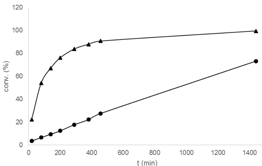
Figure 7. Reaction of \text{Ph}_2\text{SiH}_2 with acetophenone (1 mol% catalyst, d_8 -THF, rt). Conversion (%) of acetophenone vs. time, circles: complex 1 ; triangles: complex 3 .
