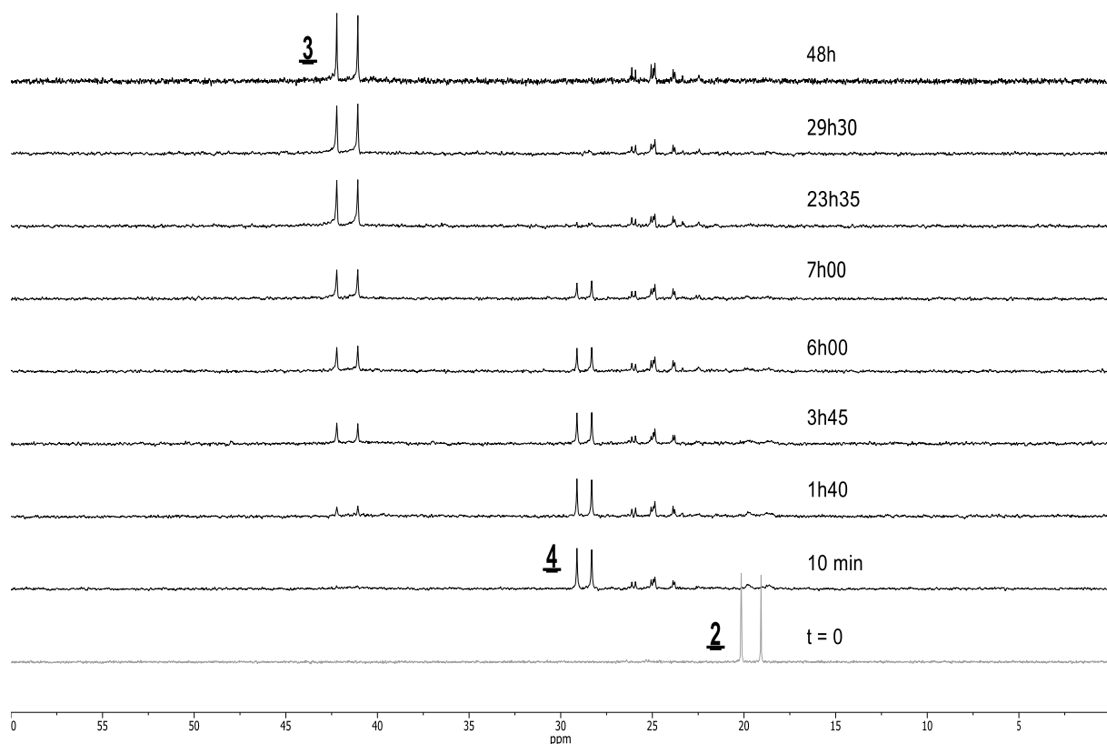
Figure 6. ^{31}\text{P} NMR spectra: oxidation of complex 2 by [\text{Th}][\text{BF}_4] in MeCN.
