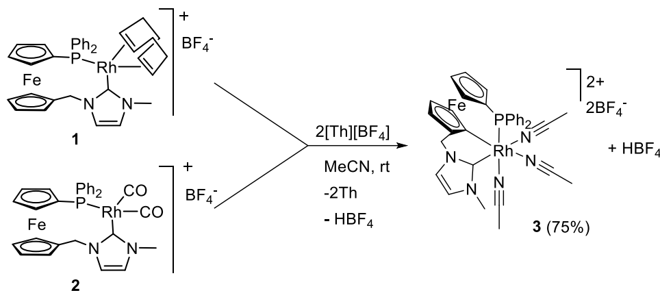
Scheme 4. Oxidation of complexes 1 and 2 with [Th][BF 4 ] in MeCN.
