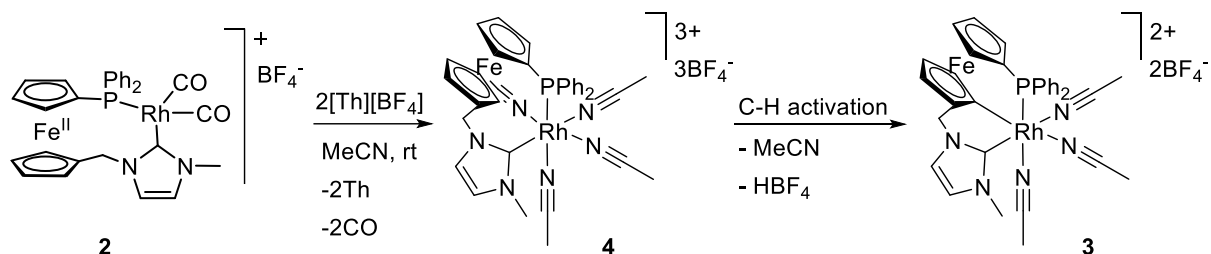
Scheme 5. Intermediate species ( 4 ) in the oxidation process of \text{Rh}^{\text{I}} complex 2 to \text{Rh}^{\text{III}} complex 3 .
