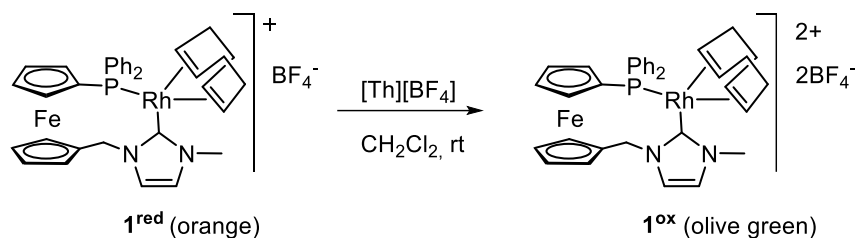
Scheme 2. Oxidation of rhodium(I) complex 1 with [\text{Th}][\text{BF}_4] in \text{CH}_2\text{Cl}_2 .
