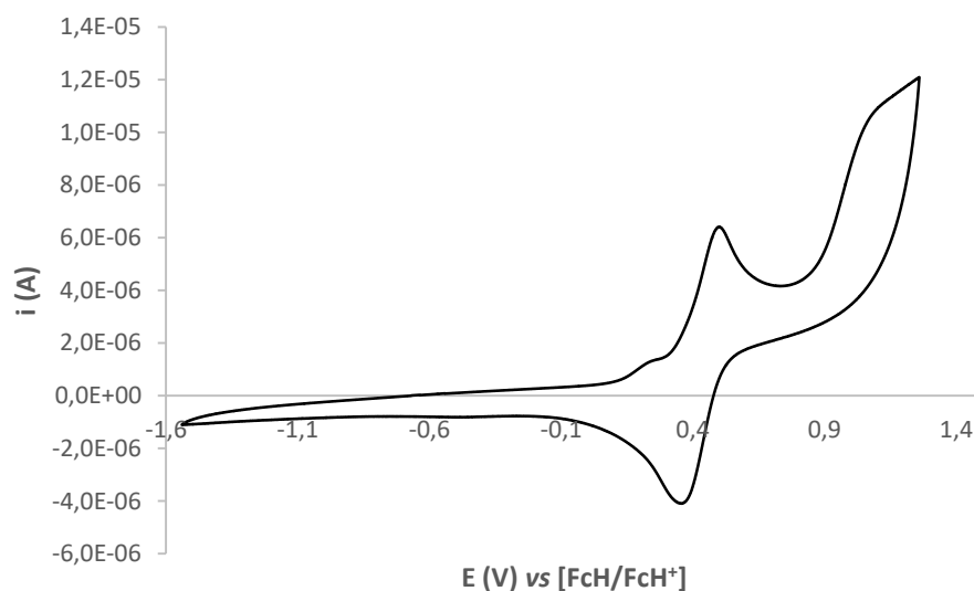
Figure 3. Cyclic voltammogram on a Pt electrode of complex 2 : 1 mM in CH 2 Cl 2 with n Bu 4 NBF 4 (0.1 M) at a scan rate of 0.2 V s -1 .
