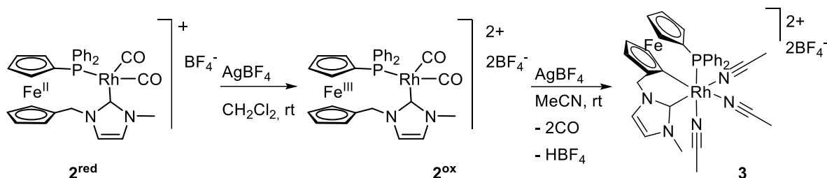
Scheme 6. Stepwise oxidation of complex 2 in \text{CH}_2\text{Cl}_2 and reaction of 2 ox in MeCN.
