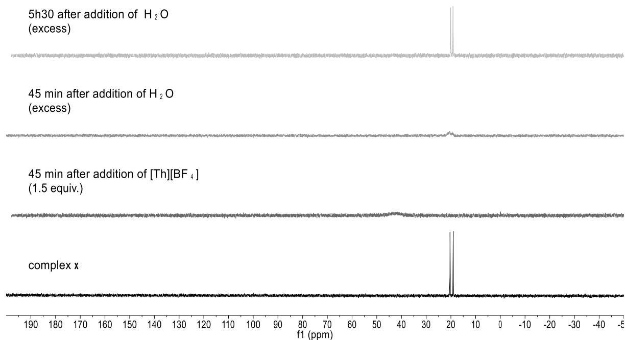
Figure 4. ^{31}\text{P} NMR spectra: oxidation of complex 1 by [\text{Th}][\text{BF}_4] in \text{CD}_2\text{Cl}_2 .
