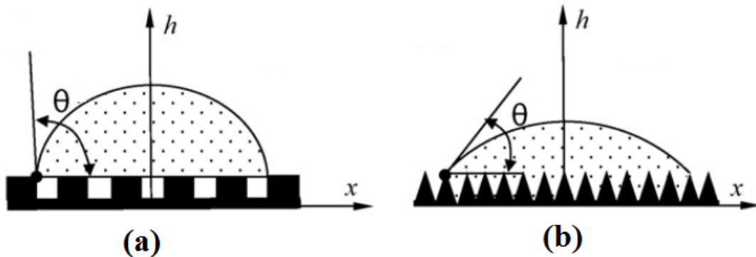
Figure 1: (a) Cassie-baxter and (b) Wenzel droplets on textured surfaces (image from [21]).
