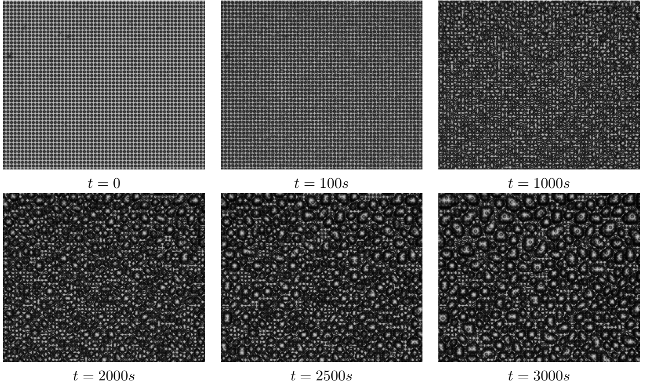
Figure 13: An example of droplets growth procedure on surface configuration 5. The first image shows the pillars just before droplets nucleation. The size of each image is 3.3mm \times 2.7mm .
