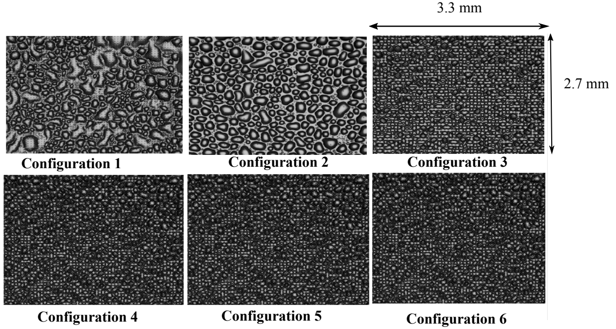
Figure 15: Illustration of 6 pillared surfaces after 1800s. The size of the substrate at each image is 3.3mm \times 2.7mm .
