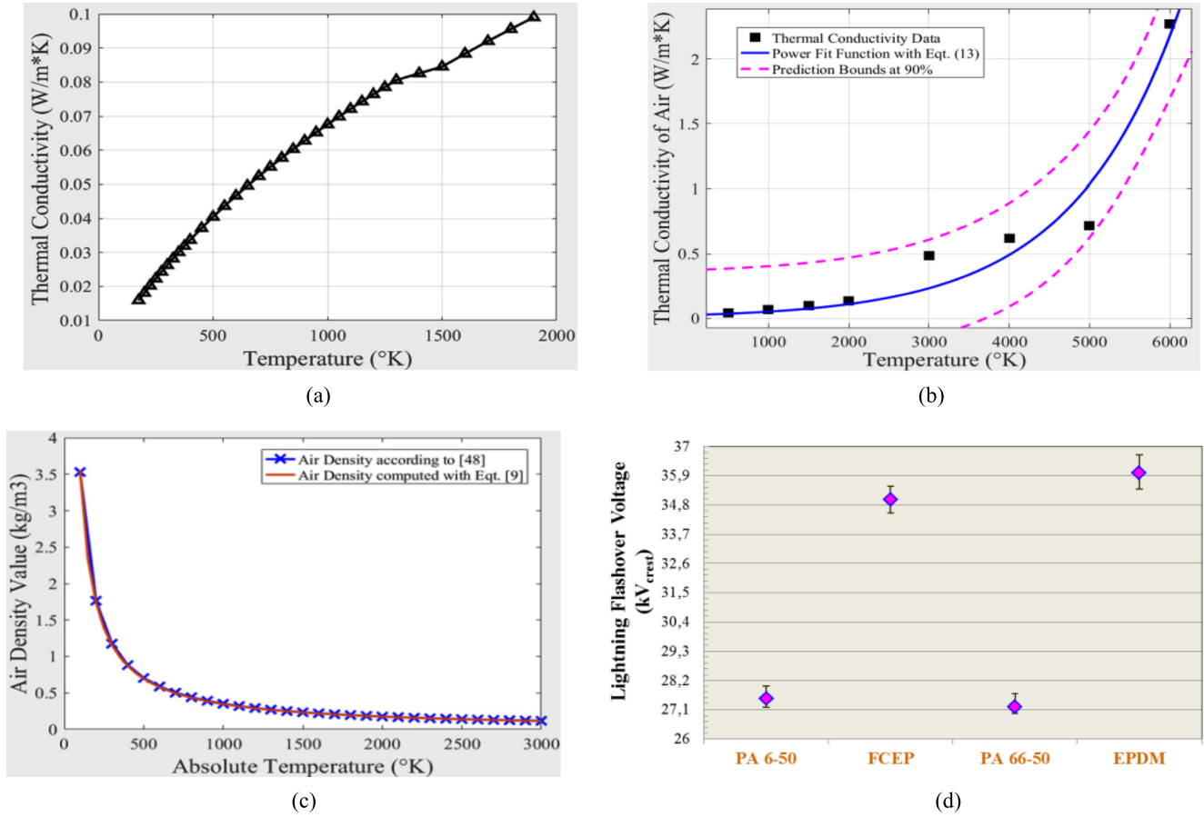
Fig. 9. Influence of temperature on atmospheric air properties ( P = 1013 kPa): (a) thermal conductivity below 2000 K; (b) modelling of thermal conductivity at higher temperature ( T \leq 6000 K); (c) air density below 3000 K [68,71,72]; and (d) crest values of flashover voltage (FOV).
