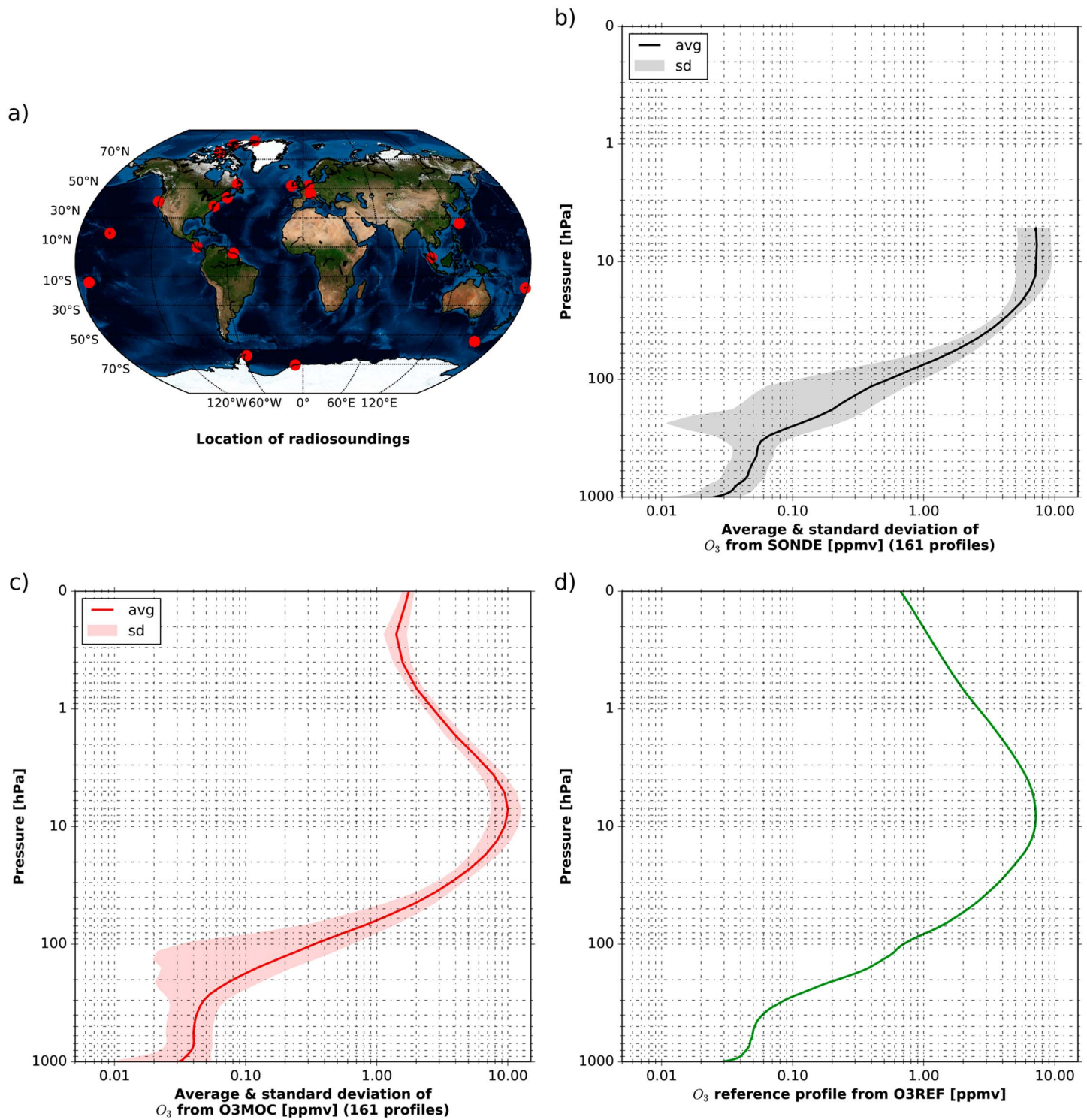
Figure 2. Location of radiosoundings from (WUOUDC, SHADOZ, and NOAA) networks used in this study (a), average and standard deviation of the 161 ozone profiles from SONDE (b), O3MOC (c), and ozone reference profile from O3REF (d) with respect to pressure.
