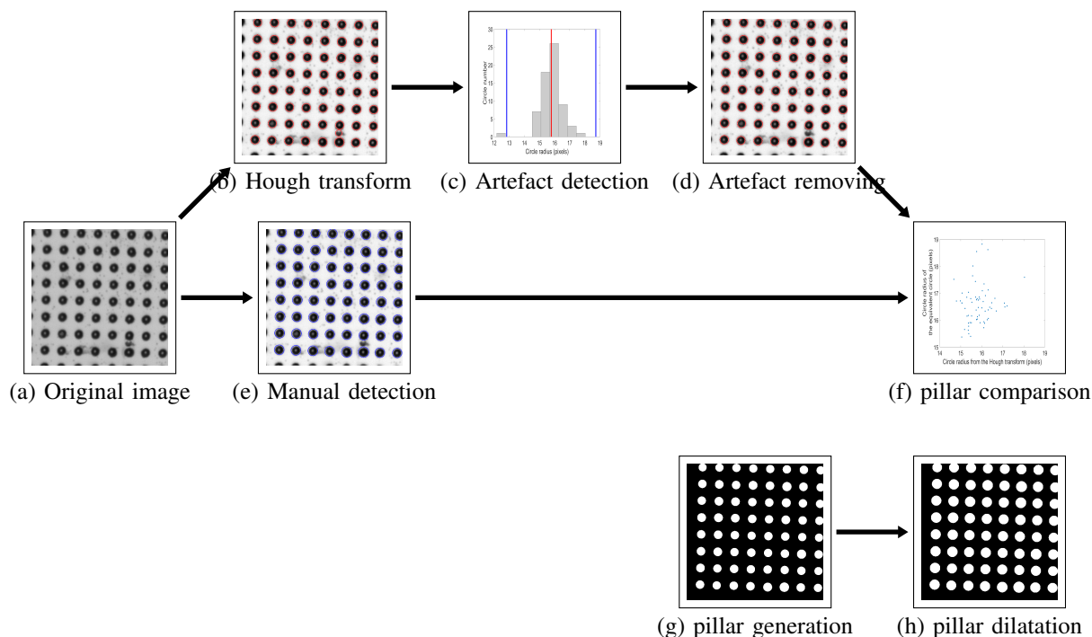
Fig. 3. Algorithm for pillar characterization
