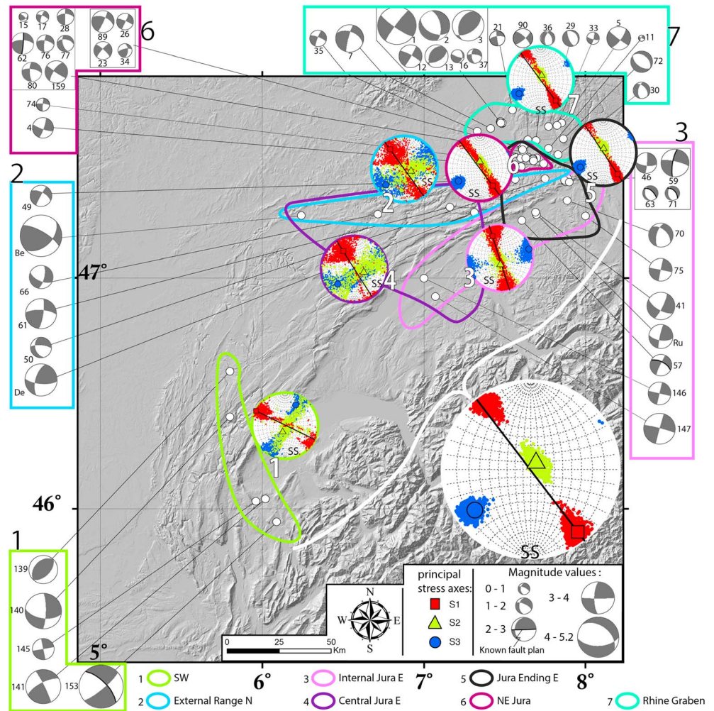
Figure 6. Results of the seismic inversions for each considered inversion zone (colored stereograms) and for the entire arc (white stereogram, right bottom angle). The three stress axes have been reported on the lower hemisphere of Wulff nets. The scattered points on each stereogram correspond to the 2,000 results of the bootstrapping method.
