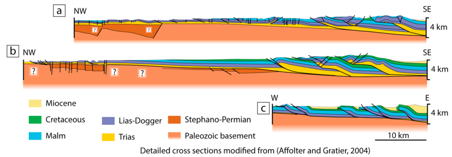
Figure 2. Schematic cross sections (modified after Affolter & Gratier, 2004) approximately relocated in Figure 1 (white lines). Question marks on cross sections represent uncertainties on the deep geometry of the basement. The three sections are detached in the Trias evaporites (Keuper).
