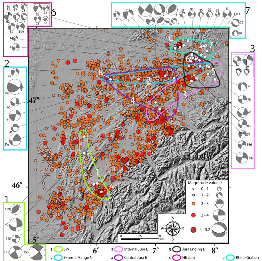
Figure 3. Seismicity of the Jura Mountain between 1971 and 2012 recorded by the French Alpine Seismic Network, the French National Seismic Monitoring Network, and the Swiss Seismological Service. The station locations of these three networks around the Jura Mountains are presented on Figure 4. The three white letters on the map correspond to the three biggest events: (a) 1996 Vuache earthquake ( M_l 5.2); (b) 2004 Besançon earthquake ( M_l 4.8); and (c) 1980 Sierentz earthquake ( M_l 4.7). The 54 focal mechanisms computed in the Jura Mountains and its vicinity between 1971 and 2015 are compiled from Kastrup et al. (2004), Baer et al. (2005), and Deichmann et al. (2006, 2012). Seven so-called inversion zones have been determined based on the spatial distribution of mechanisms and structural pattern of the arc (numbered and colored shapes on the map, zones 4 and 5 include focal mechanisms of zones 2 and 3 and 2, 3, and 6, respectively).
