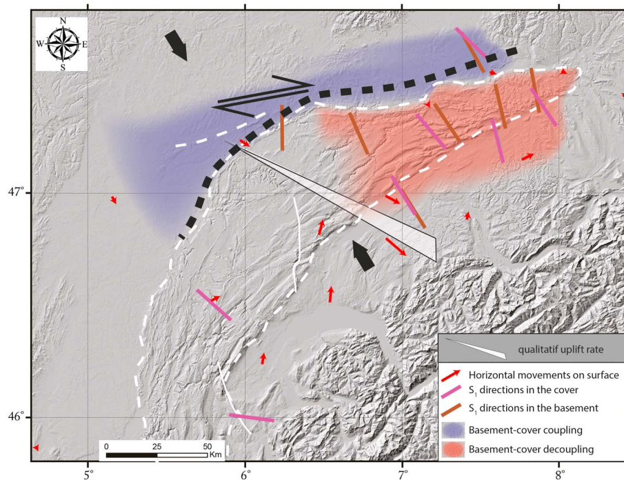
Figure 16. Interpretative map of the current deformation of the Jura and its vicinity. In the eastern part of the Jura, the cover seems to be decoupled from the basement while they seem coupled at the front of the Jura, in the Rhine-Bresse Transfer Zone. The extent of these two deformation modes in the central part of the Jura and in its western part is not enough constraint by available data and has not been represented here. The entire Alpine Foreland represented by the folded Jura, the Molasse Basin, and the front of the Jura is affected by a general uplift increasing toward the Alpine front where it reaches \sim 0.4 mm/year, which is in linear continuity with the uplift observed in the Alps (e.g., Nocquet et al., 2016, see text for details).
