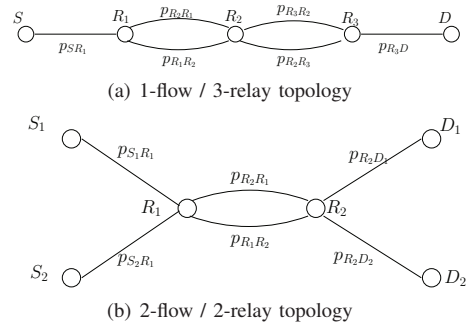
Fig. 1. Investigated topologies: (a) Linear topology composed of one flow and 3 relay nodes ; (b) Crossflow topology with 2 flows.
