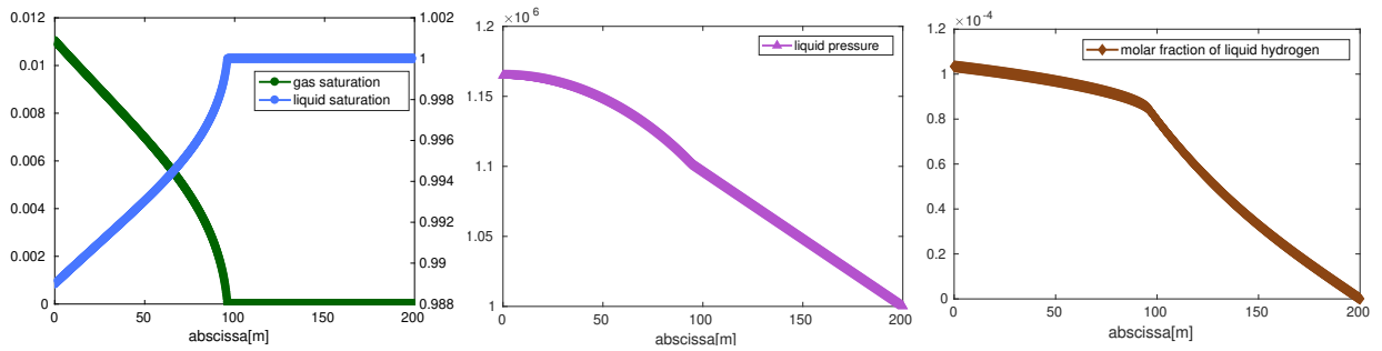
Figure 1: Solution at convergence ( k = \bar{k} , i = \bar{i} ) for N_{\text{sp}} = 1000 elements at t = 1.05 \times 10^5 years. Left: saturation of the phases, middle: pressure of the liquid phase, right: molar fraction of liquid hydrogen.
