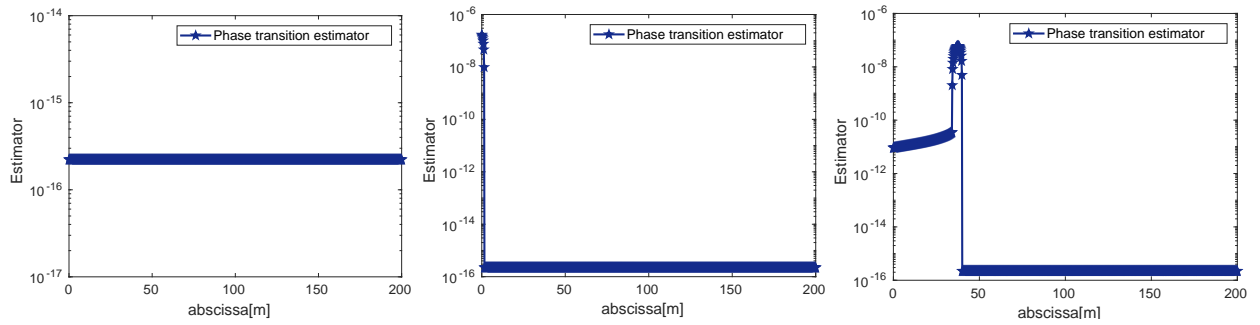
Figure 3: Phase transition estimator \eta_{P,K,\text{pos}}^{n,k,i} at convergence ( k = \bar{k}, i = \bar{i} ). Left: one-phase liquid. middle: appearance of gas phase, right: two-phase liquid-gas.
