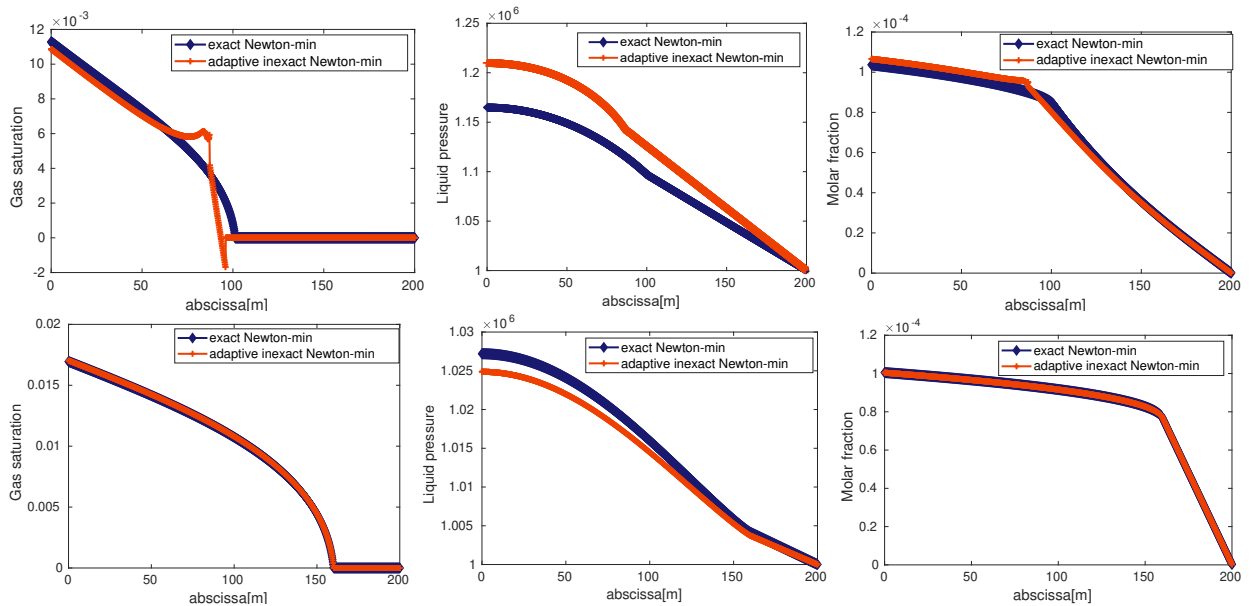
Figure 8: Gas saturation (top left), liquid pressure (top middle), and molar fraction of liquid hydrogen (top right) for exact Newton-min and adaptive inexact Newton-min at convergence at t = 1.05 \times 10^5 years. Gas saturation (bottom left), liquid pressure (bottom middle), and molar fraction of liquid hydrogen (bottom right) for exact Newton-min and adaptive inexact Newton-min at convergence at t = 3.5 \times 10^5 years.
