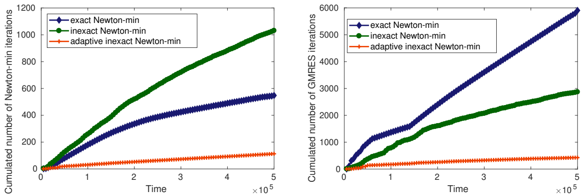
Figure 7: Cumulated number of Newton-min iterations as a function of time (left), and cumulated number of GMRES iterations as a function of time (right).
