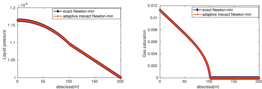
Figure 9: Liquid pressure (left) and gas saturation (right) for exact Newton-min and adaptive inexact Newton-min at convergence at time t = 1.05 \times 10^5 years with \gamma_{\text{alg}} = 10^{-3} and \gamma_{\text{lin}} = 10^{-6} . The two curves superimpose.
