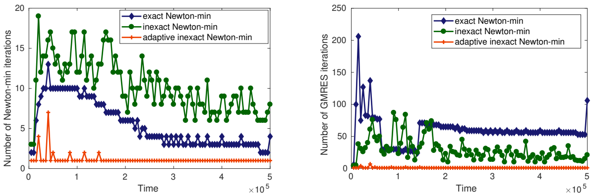
Figure 6: Number of Newton-min iterations at each time step (left), number of GMRES iterations at each time step (right).
