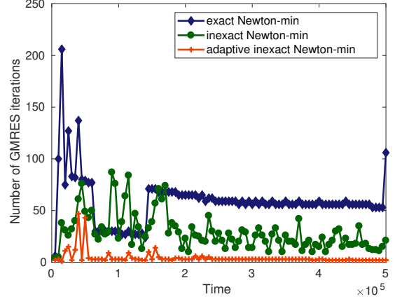
Figure 6: Number of Newton-min iterations at each time step (left), number of GMRES iterations at each time step (right).
