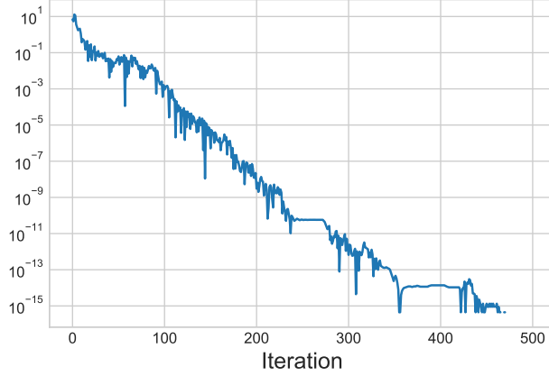
Figure 9: |x_n - g_n| over 500 iterations in a logarithmic scale. After 300 iterations, we reach the computer precision. One can notice the linear behavior of \log(|x_n - g_n|) .
