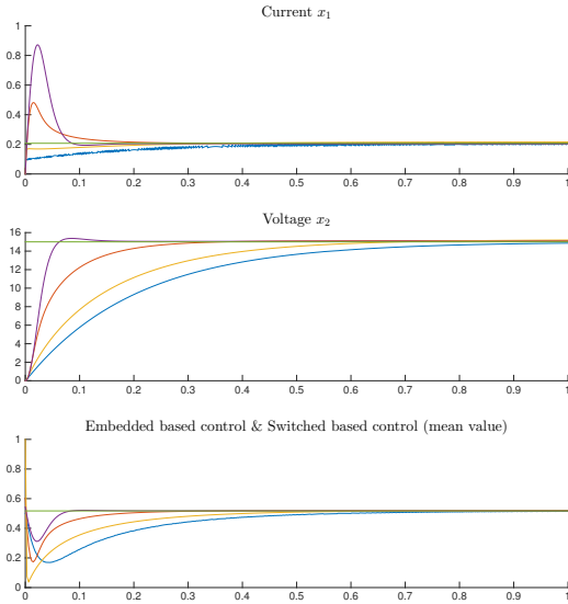
Fig. 6. Start-up transient: Plot 1 shows the current x_1 , Plot 2 shows the voltage x_2 . Plot 3 shows the control (in average for the switched based control case). Switched based control (Blue); Embedded based control (Purple, k_1 = 3.10^{-7} ) (Red, k_1 = 1.10^{-6} ) (Yellow, k_1 = 7.10^{-6} ). Time is given in (ms).
