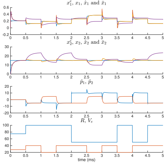
Fig. 7. Plot 1 shows respectively the current reference (Blue), the current x_1 (Yellow) when the adaptive embedded control \lambda is used, its estimation \hat{x}_1 (Red) and the current \bar{x}_1 (Purple) when only the embedded based control \lambda is used without load and input estimation. Time is given in (ms). Plot 2 shows the voltage x_2 using the same convention. Plot 3 shows the variation of the estimated value \hat{p}_1 (respectively \hat{p}_2 ) of parameter p_1 ( p_2 ). Finally, Plot 4 shows the load R and input V_e variations.
