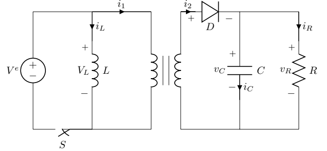
Fig. 1. A Flyback converter
