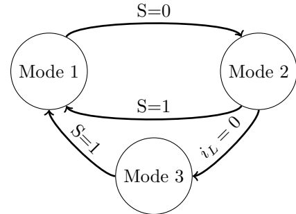
Fig. 2. Flyback modes and switching rules
