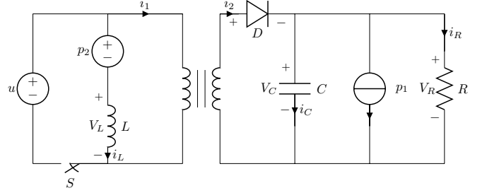
Fig. 5. Flyback converter with parameters estimation
