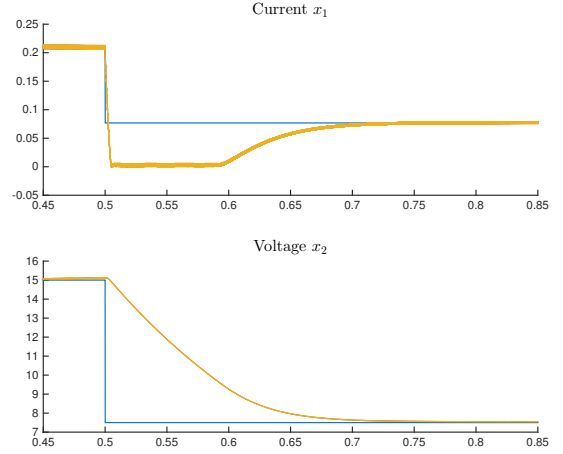
Fig. 8. DCM transient. Plot 1 shows the current x_1 (yellow), Plot 2 shows the voltage x_2 (yellow) when a step variation of the reference (blue) leads to DCM mode.
