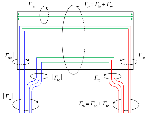
Figure 3. Schematic shows the circulations associated with a finite wing with reattached flow. \Gamma_0 is the effective bound circulation, \Gamma_{le} is the circulation of the vortices representing the LESR; the dots represent that they are bound to the wing. \Gamma_{te} is the circulation shed at the trailing edge, \Gamma_{se} is the circulation shed at the side edges (wing tips) and \Gamma_w is the circulation of the fully formed wake vortices. (Online version in colour.)
