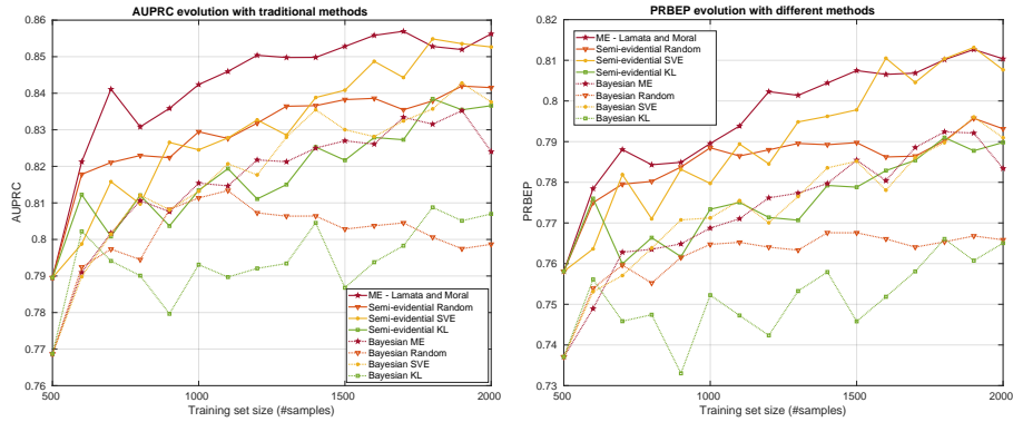
Figure 5: AUPRC and PRBEP at every iteration. Comparison of evidential-based disagreement measures with traditional ones.
