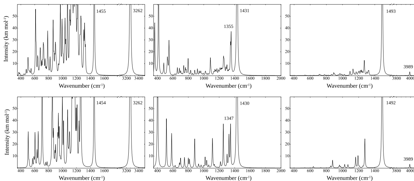
Fig. 2 B3LYP simulated IR spectra of the \text{VN}_3\text{H} (left), \text{I}_{2\text{N}} (center) and \text{VH}_4 (right) defects obtained with the FHD (top) and the fragment (bottom) strategies. The big fragment, BF, has been used. Values refer to the \text{S}_{216} supercell.
