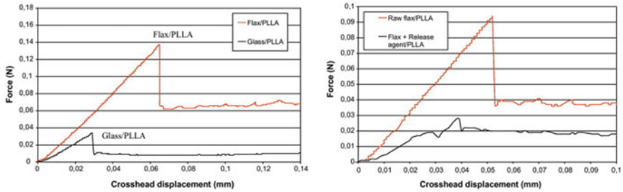
Fig. 5.5 Typical microdroplet test plots for flax/PLLA and de-sized E-glass/PLLA (left); Influence of release agent on microdroplet test for flax/PLLA (right). Reprinted from (Le Duigou et al. 2012) with permission from Elsevier
