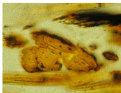
B=Discoloured fibre bundle (onset of thermal damage: mid degradation region)
