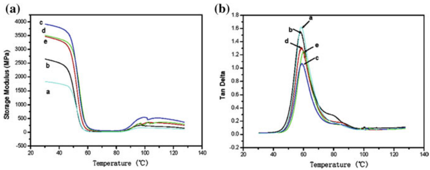
Fig. 5.19 Temperature dependence of storage modulus (A) and damping factor (B) of PLA and PLA-based composites: neat PLA (a), composite with untreated fibres (b), composite with alkali treated fibres (c), composite with APS silane treated fibres (d), composite with GPS silane treated fibres (e). Reprinted from Yu et al. (2010), Fig. 5 with permission from Elsevier
