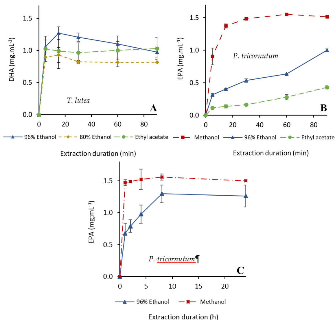
Figure 3. Kinetics of extraction of docosahexaenoic acid (DHA) from T. lutea (A) and eicosapentaenoic acid (EPA) from P. tricornerutum (B) with ethanol (80 or 96%), methanol (100%) and ethyl acetate (100%). Extractions were carried out from freeze dried biomass for 90 min at 30 °C (A,B) and for 24 h at 40 °C (C) with a 20:1 ( v/w ) solvent/biomass ratio in a closed system with magnetic stirring ( n = 3 replicates).
