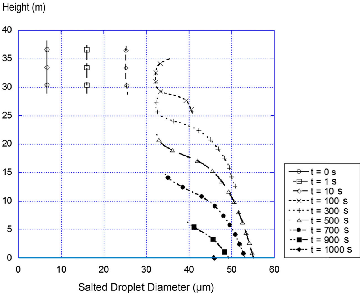
FIG. 6. Salted droplet diameter vs height and time for run 1.
