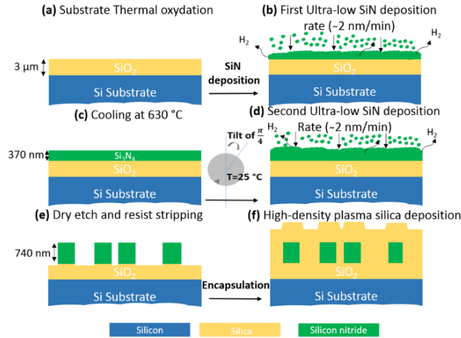
FIG. 1. Schematics of the annealing-free fabrication process for Si 3 N 4 nonlinear photonics (a)-(f).
