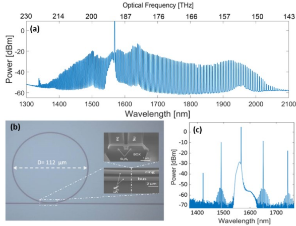
FIG. 3. Comb generation using annealing-free silicon nitride on insulator. (a) A 800-nm-spanning comb generation using a 56- \mu\text{m} -radius \text{Si}_3\text{N}_4 microresonator for coupled power P_{\text{in}} \sim 1 W. (b) Optical microscope and (insets) scanning electron microscope images of the ring and coupling region. (c) Comb spectrum for P_{\text{in}} \sim 300 mW.
