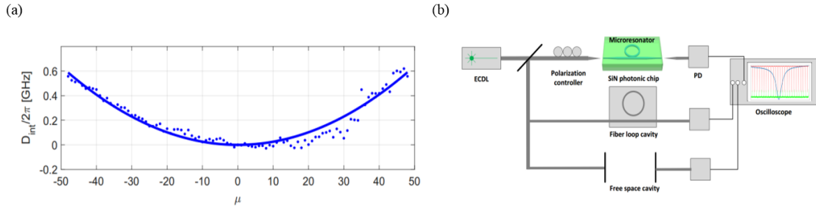
FIG. 4. Dispersion measurement of the TE mode of a ring resonator with 200 \mu\text{m} radius and 1.5 \mu\text{m} width. (a) Plot of the integrated dispersion. (b) Experimental setup used for the dispersion measurement.
