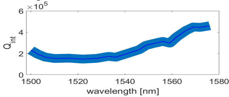
FIG. 2. Intrinsic quality factor as a function of wavelength for an annealing-free silicon nitride microring resonator (waveguide width equal to 1.4 μm). The darker colored line shows the mean value and the brighter shadowed areas illustrates the standard deviation of the measurements.
