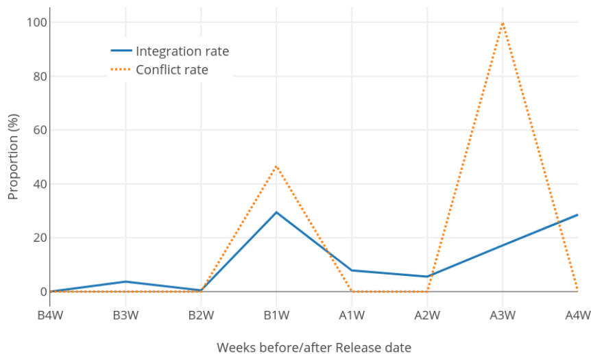
Fig. 2 IkiWiki-V3.0, integration and conflict rate on files
