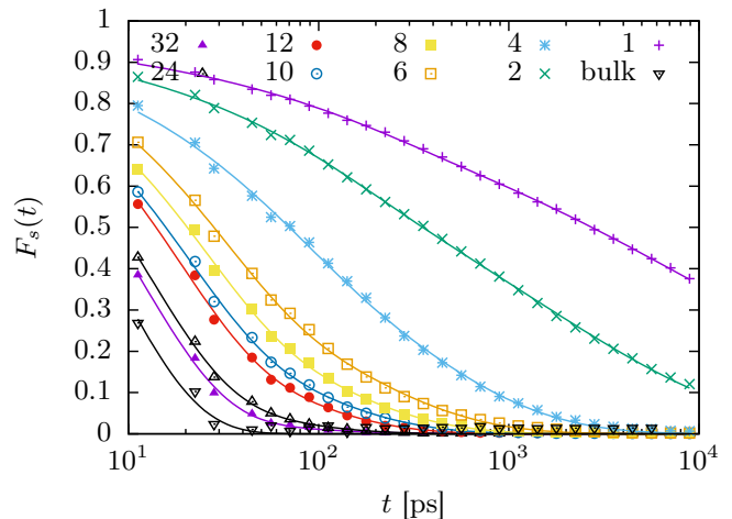
FIG. 5. The self-intermediate scattering functions, F_s(q, t) , calculated from the oxygen atoms of the water molecules via Eq. (3) (symbols). These data correspond to q^* = 0.7 \text{\AA}^{-1} , at the indicated values of \lambda . We also show as solid lines the best-fits to the data, according to Eq. (4). These results strongly support the hypothesis of the existence of two dynamical populations, as discussed in details in the main text.
