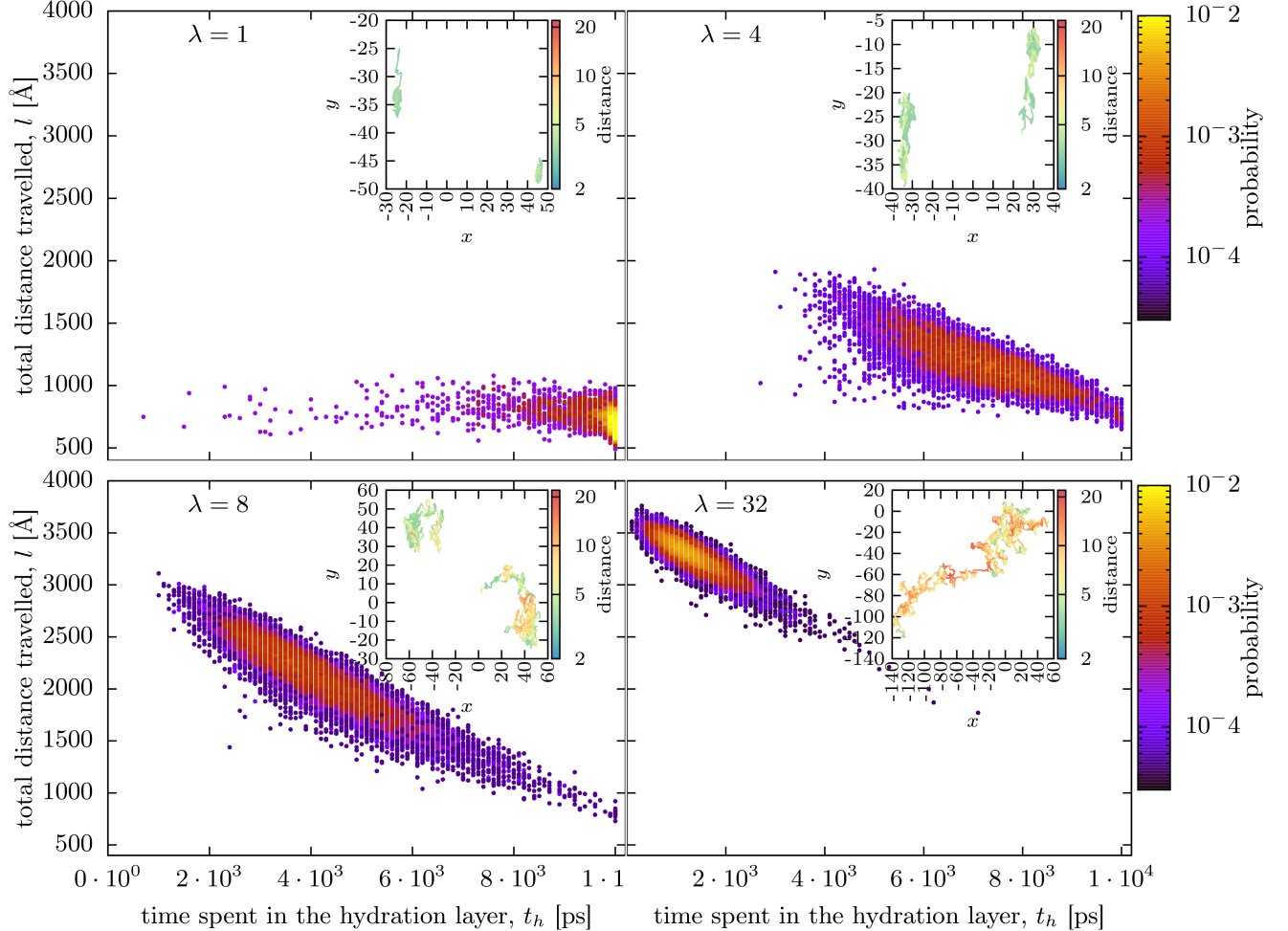
FIG. 11. Joint probability distribution of the total displacement, l , of water molecules on the entire time scale of the run, \tau_{\max} , and the total time, t^h , they have spent (even discontinuously) in the hydration layer of a surfactant head, on the same time window. The probability is represented as colour maps, for the indicated values of \lambda : yellow indicates high probability, indigo lower. In the insets we show the projection on the xy -plane of the trajectory followed by two molecules chosen at random at the corresponding \lambda , with the incremental distance travelled at each time indicated by the displayed colour code.
