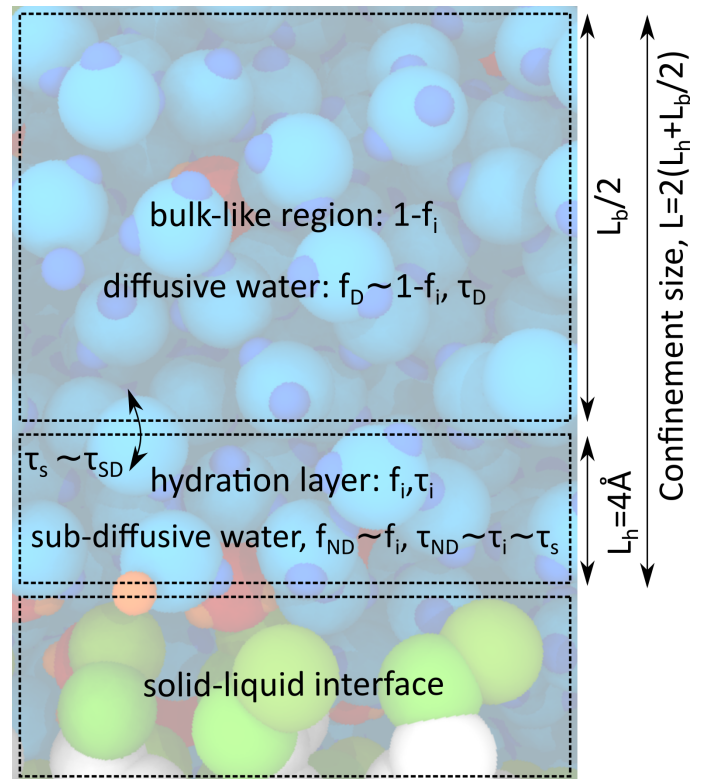
FIG. 10. Schematic overview of the interplay between the structure of the surfactant phase and the transport properties of the confined water molecules. This sketch complements the detailed discussion contained in the main text.
