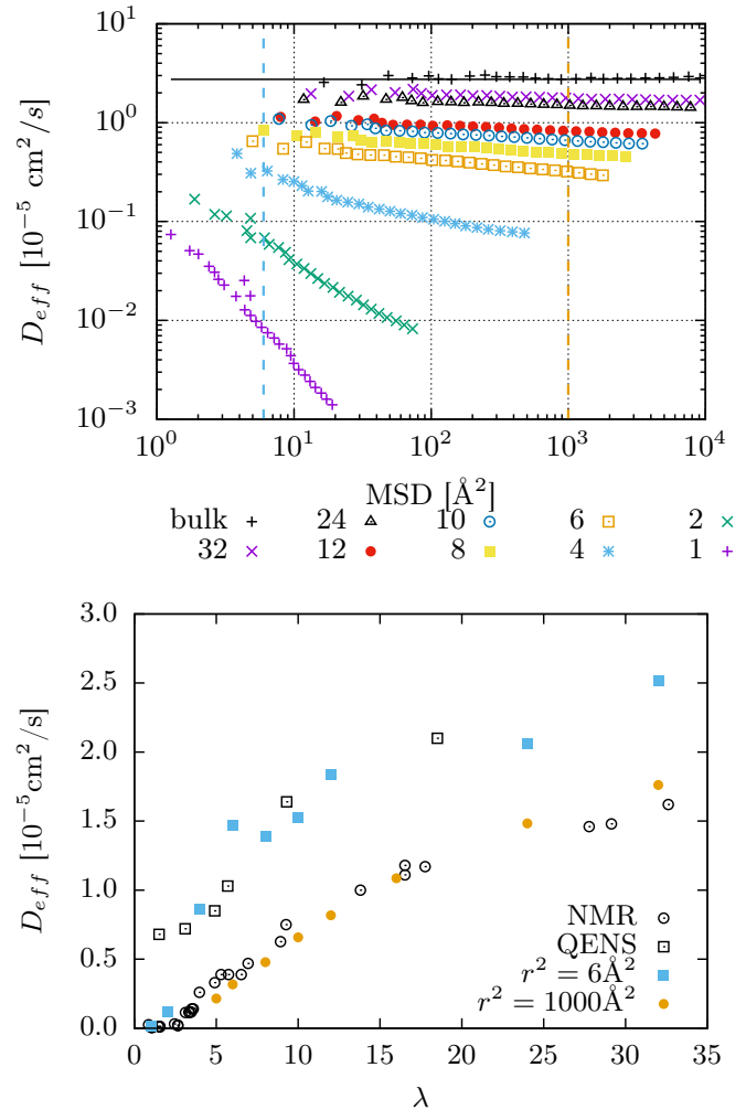
FIG. 4. Top: The effective diffusion coefficient, D_{\text{eff}} , computed from Eq. (2), plotted parametrically against \langle r^2(t) \rangle . The solid black line is the result in the bulk for the considered water model, corresponding to D \simeq 2.74 \times 10^{-5} \text{ cm}^2/\text{s} . The dashed vertical lines, indicate the (squared) length scales \simeq 6 and \simeq 1000 \text{ \AA}^2 used to select the values of D_{\text{eff}} shown in the bottom panel, as discussed in the text. Bottom: The values for D_{\text{eff}} selected by the two verticals lines of the above panel are shown as closed symbols. We also show the diffusion coefficients obtained by PFG-NMR and QENS spectroscopy [23], which probe the dynamics on long and short length scales, respectively.
