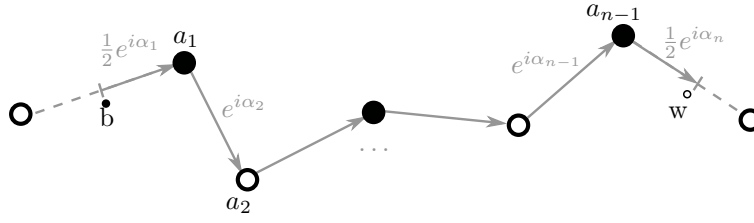
Figure 18: A path on \mathcal{Q} from b to w .
