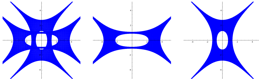
Figure 2: Amoebas of the curves defined by P_{\alpha, \beta}^{8V} , P_{\alpha}^{6V} and P_{\beta}^{6V} for the square lattice.
