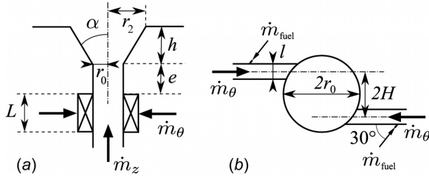
Fig. 2 Sketch of the injector: (a) axial cut and (b) transverse cut through the swirler
