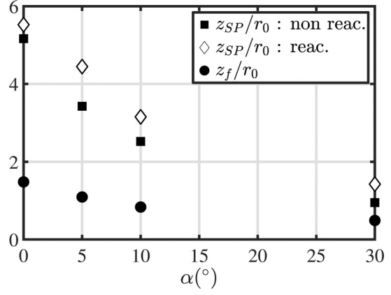
Fig. 6 Internal recirculation zone leading edge position z_{SP}/r_0 in nonreacting (black squares) and reacting (empty diamonds) flow conditions, and flame leading edge position z_f (black disks) as a function of the injector diffuser cup angle \alpha
