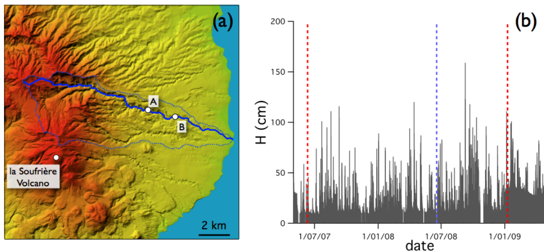
Figure 1 (a) Topographic map of the Capesterre watershed. The frontiers of the watershed and the Capesterre river are indicated by respectively the dotted and the solid curve. The suspended load sensor is located on site A while the drone imaging method was tested on site B. (b) Variations of the water flow depth in the Capesterre river on site A between june 2007 and june 2009 (data by courtesy of the Direction Régionale de l'Environnement). The dates of image acquisition (06/11/2007 and 01/09/2009) are indicated by the two red vertical dotted line. The installation date of the suspended load sensor (06/18/2008) is indicated by the vertical dotted blue line.
