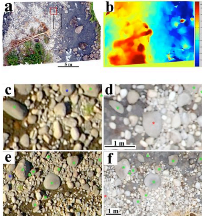
Figure 5 Example of ortho-images of a gravel bank of the Capesterre river showing the change of granulometry which occurred between January 2008 to January 2009. a) and b) General view and Digital Elevation Model of the studied gravel bank in 2009. The squares show the position of the high resolution ortho-images shown in c) d) (red square) and e) f) (black square). The images c) and e) are from 2008. The images d) and f) are from 2009. Green stars indicates the boulders which have not moved, blue stars on 2008 images indicate the largest boulder which were taken away during the floods, red stars on 2009 images show the largest boulders which were deposited by the flood.
