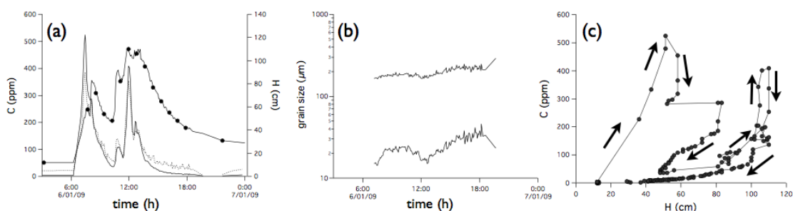
Figure 4 Data acquired by CAPMES during a flash flood on January 6th 2009. (a) Water flow depth (line with circles), volumetric concentration of suspended silt (solid line) and sand (dotted line) as a function of time; (b) Average grain size of silt and sand particles as a function of time; (c) Plot of silt concentration vs water level. Arrows indicate forward time.
