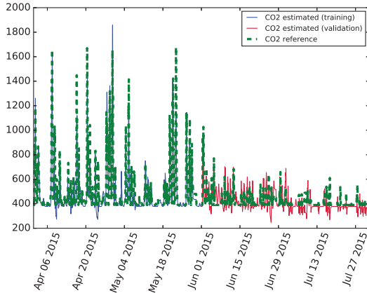
Figure 9: CO 2 concentration of the ARX model inspired by physics
