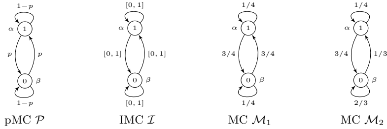
Fig. 10: pMC \mathcal{P} , IMC \mathcal{I} , MC \mathcal{M}_1 , and MC \mathcal{M}_2 s.t. \mathcal{M}_1 \models_{\mathcal{P}} \mathcal{P} and \mathcal{M}_1 \models_{\mathcal{I}}^a \mathcal{I} but \mathcal{M}_2 \not\models_{\mathcal{P}} \mathcal{P} and \mathcal{M}_2 \not\models_{\mathcal{I}}^a \mathcal{I} while \mathcal{P} is entailed by \mathcal{I}
