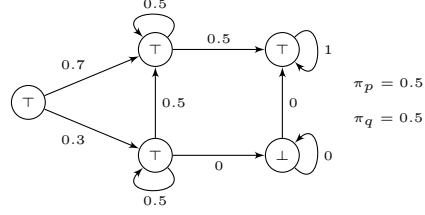
Fig. 6: Variables in the CSP produced by \mathbf{C}_{\exists c} for the pIMC \mathcal{P} from Fig. 5 Fig. 7: A solution to the CSP \mathbf{C}_{\exists c}(\mathcal{P}) for the pIMC \mathcal{P} from Fig. 5
