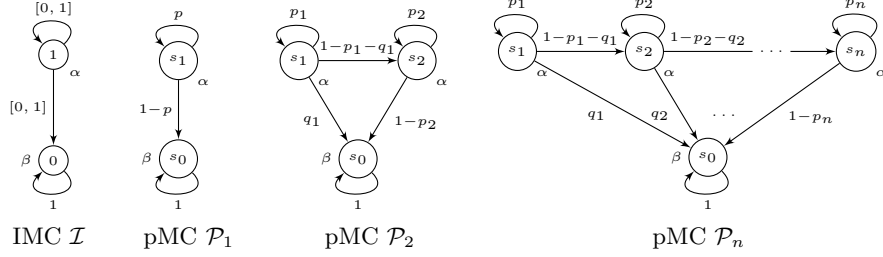
Fig. 9: IMC \mathcal{I} with three pMCs \mathcal{P}_1 , \mathcal{P}_2 , and \mathcal{P}_n entailed by \mathcal{I}
