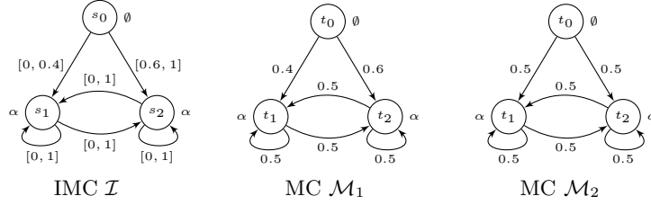
Fig. 8: IMC \mathcal{I} , MCs \mathcal{M}_1 and \mathcal{M}_2 s.t. \mathcal{M}_1 \models_{\mathbb{I}}^a \mathcal{I} and \mathcal{M}_1 \models_{\mathbb{I}}^o \mathcal{I} ; \mathcal{M}_2 \models_{\mathbb{I}}^a \mathcal{I} and \mathcal{M}_2 \not\models_{\mathbb{I}}^o \mathcal{I} the graph representation of \mathcal{I} , \mathcal{M}_1 , and \mathcal{M}_2 are isomorphic;
