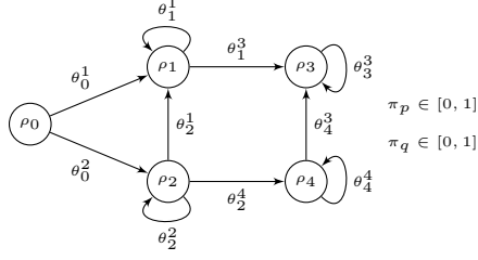
Fig. 6: Variables in the CSP produced by \mathbf{C}_{\exists c} for the pIMC \mathcal{P} from Fig. 5 Fig. 7: A solution to the CSP \mathbf{C}_{\exists c}(\mathcal{P}) for the pIMC \mathcal{P} from Fig. 5
