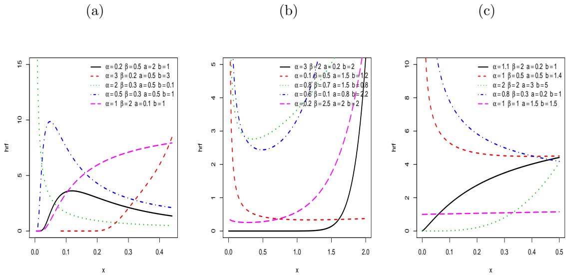
Figure 2: Plots of hrfs of the GGFr (a), GGW (b) and GGLx (c) distributions.
