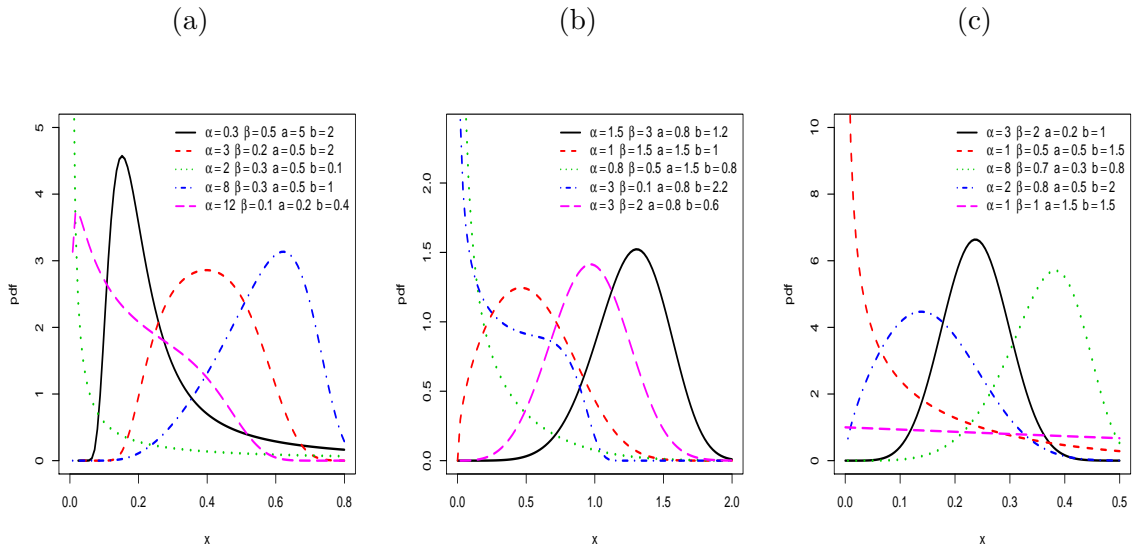
Figure 1: Plots of pdfs of the GGFr (a), GGW (b) and GGLx (c) distributions.
