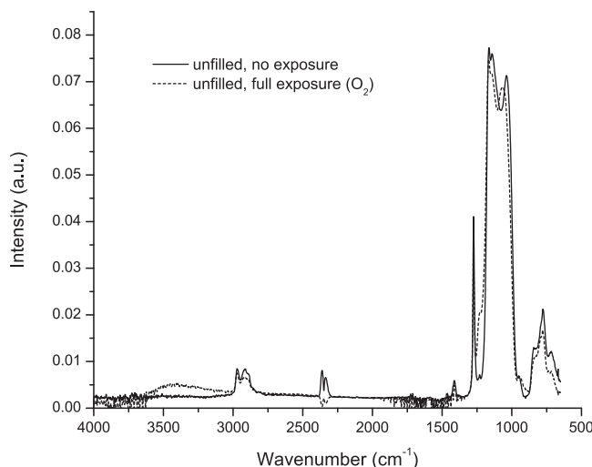
FIG. 3. Comparative FTIR spectra of the pristine and the fully exposed (O 2 ) porous dielectric material.
