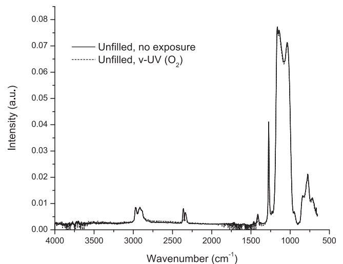
FIG. 2. Comparative FTIR spectra of the pristine and the v-UV exposed (O 2 ) porous dielectric material.
