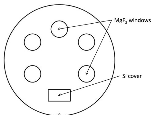
FIG. 1. Experimental wafer setup for plasma treatments.
