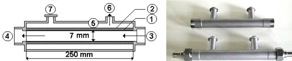
Fig. 6. Tubular pervaporation device.
