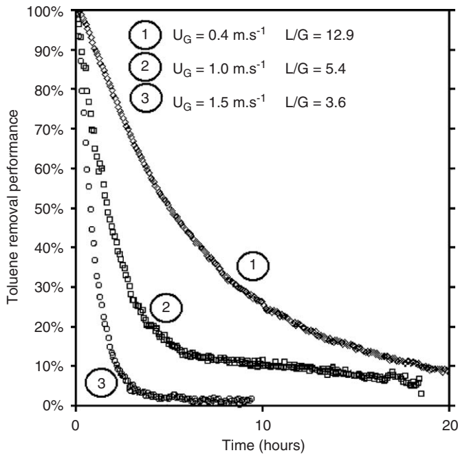
Fig. 5. Toluene removal performance as a function of time and gas superficial velocity ( L = 6.58 \text{ kg s}^{-1} \text{ m}^{-2} ).
