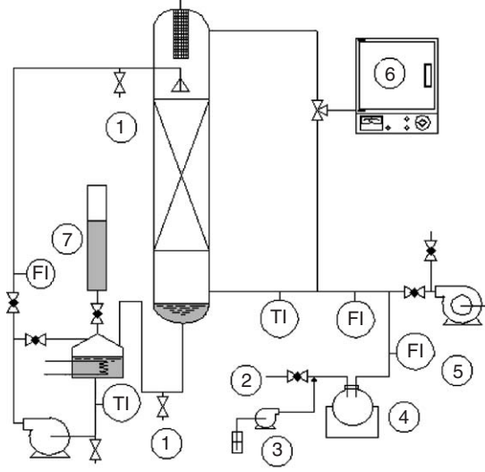
Fig. 3. Flow sheet and picture of mass transfer experimental setup.
