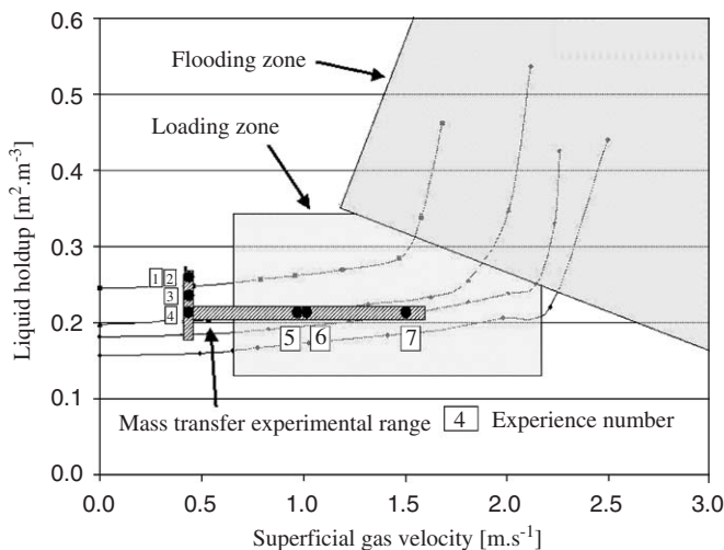
Fig. 8. Mass transfer experimental conditions and hydrodynamic zones.
