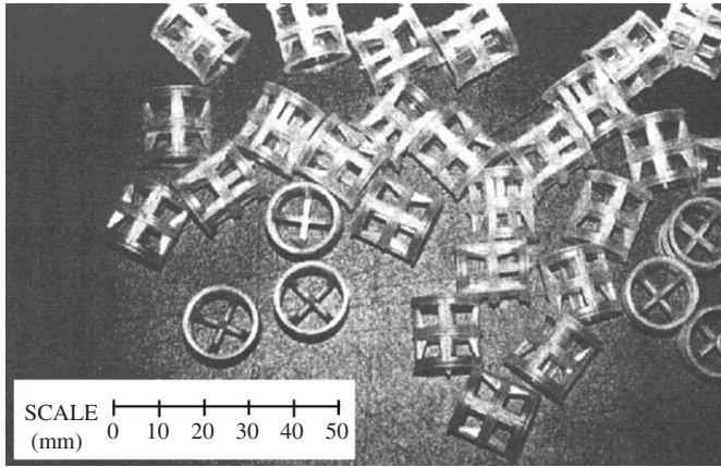
Fig. 2. Hiflow rings.
