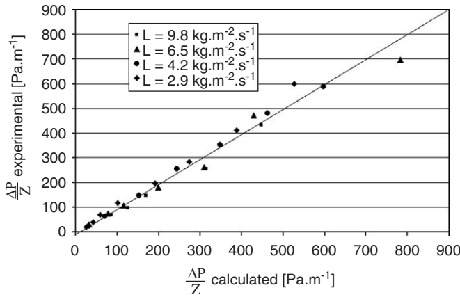
Fig. 6. Parity graph of Billet's formulae.
