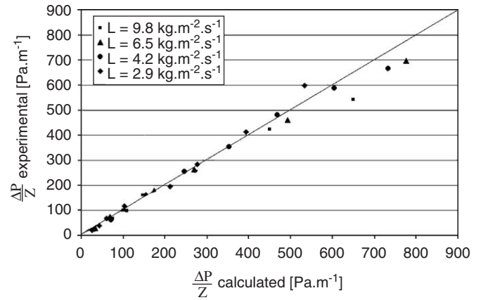
Fig. 7. Parity graph of Mackowiak's formulae.
