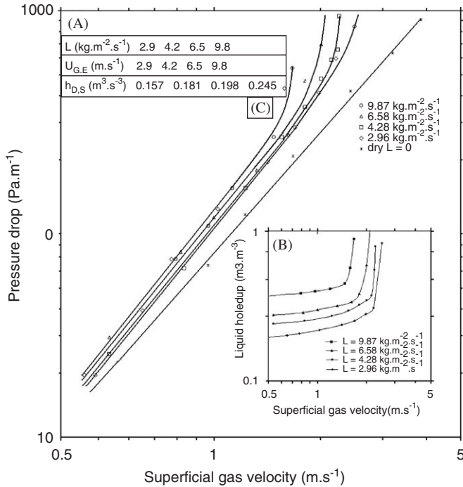
Fig. 4. Pressure drop, liquid hold-up and flooding points as a function of gas and liquid flow rates.
