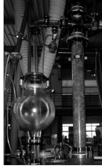
Fig. 3. Flow sheet and picture of mass transfer experimental setup.
