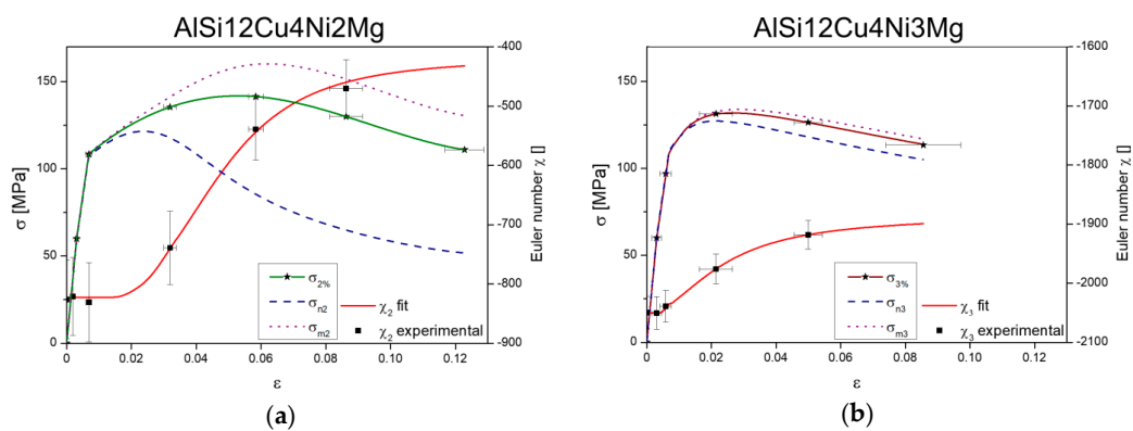
Figure 13. Evolution of stresses in the network and matrix calculated taking into account the disintegration of the 3D rigid networks by damage accumulation: (a) AISi12Cu4Ni2Mg and (b) AISi12Cu4Ni3Mg.
