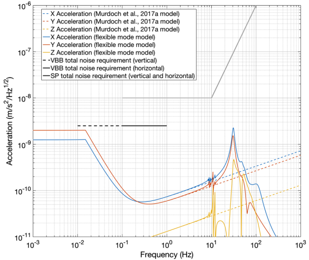
Fig. 9 Model comparison—the lander mechanical noise signal on SEIS as calculated using the inelastic lander structure model of Murdoch et al. (2017a) (dashed coloured lines), and using the new lander flexible mode model presented here (solid coloured lines). The baseline parameters for this study, as presented in Sect. 2 and Sect. 3 were used. The total noise requirements for the seismic sensors are provided in black for the VBB sensors and grey for the SP sensors
